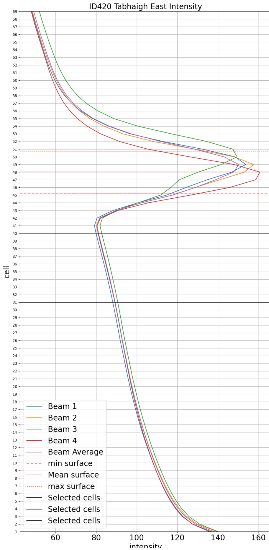
Figure 2. Mean intensity of the ADCP signal for the ID420 dataset plotted by bin number
