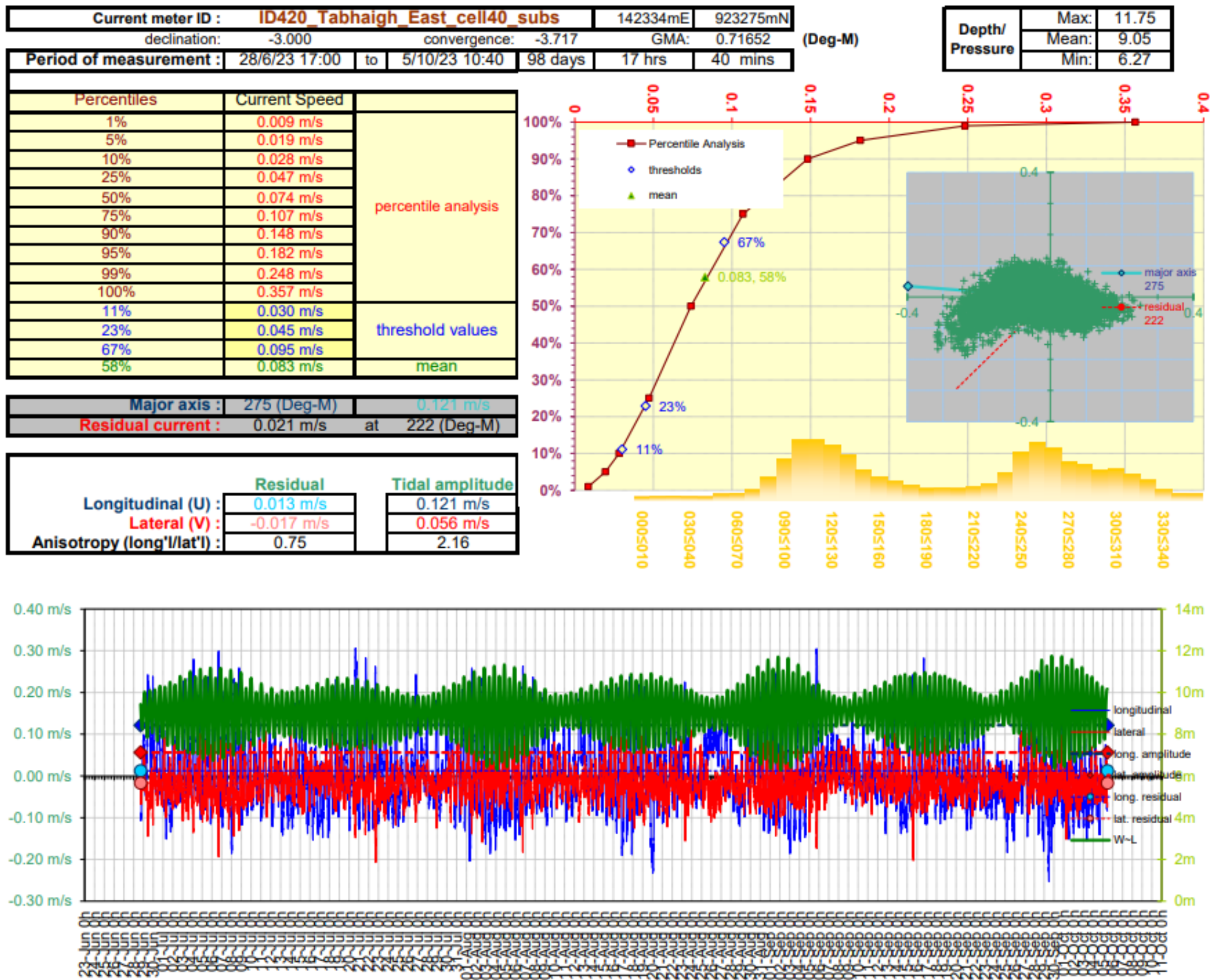
Figure 3. Current Data Summary Sheet for the surface current cell 40, 42.72 m from seabed, 28 th June 2023 to 5 th October 2023 inclusive (ID420).
