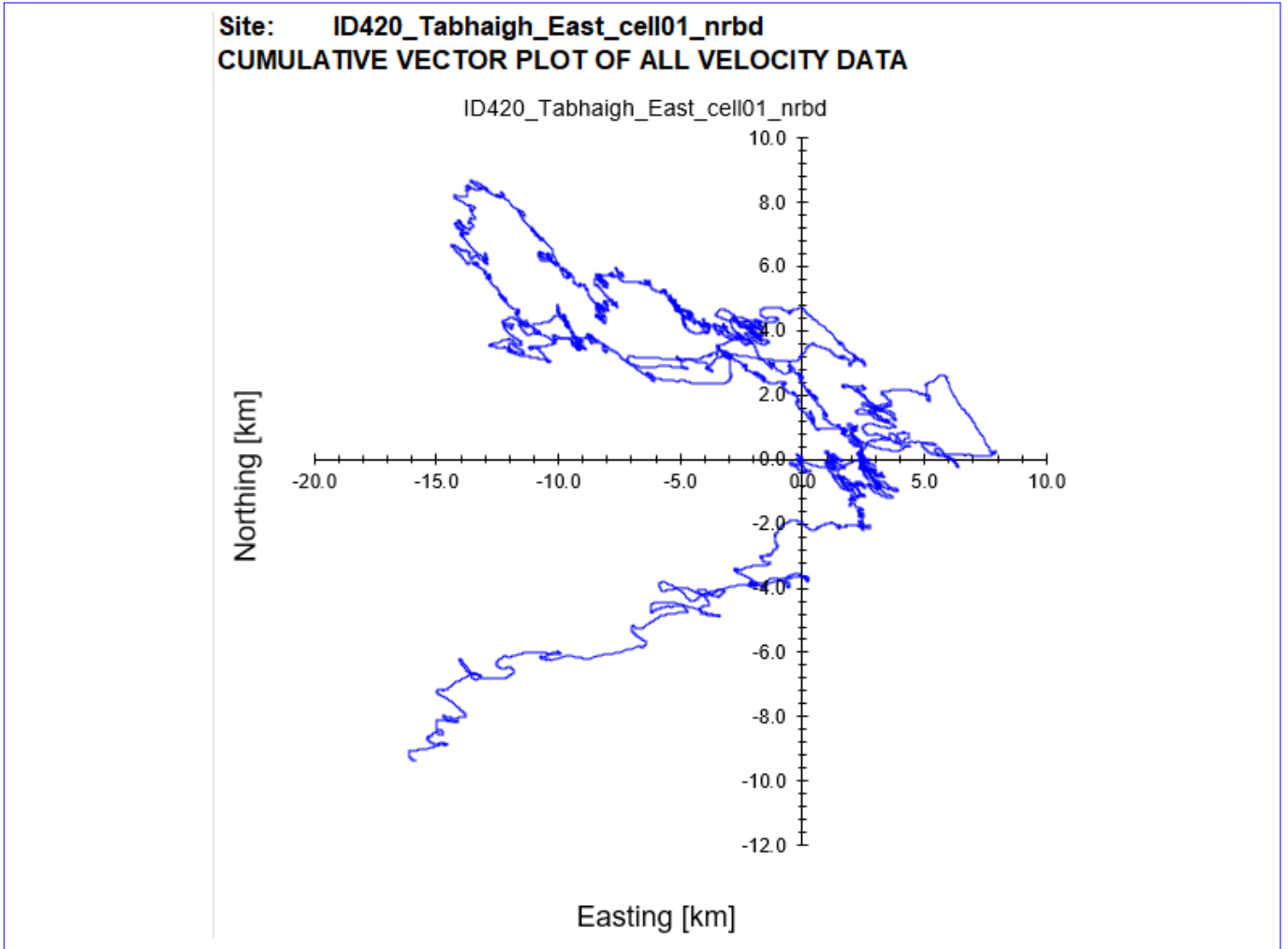
Figure 8. Cumulative Vector Plot of all velocity data from near bottom cell for ID420.
