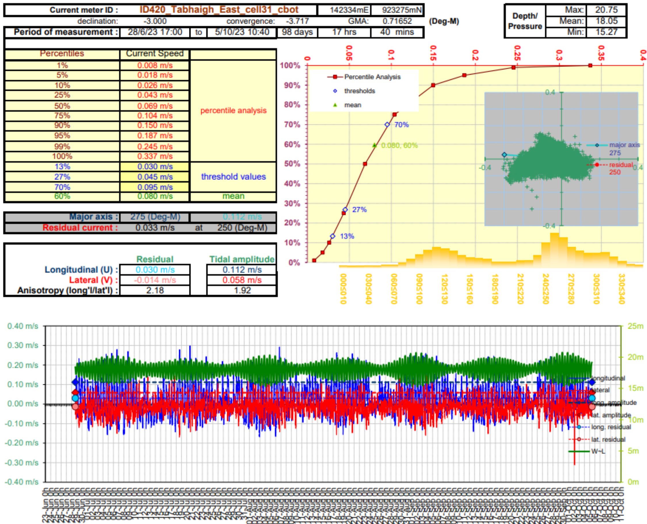
Figure 4. Current Data Summary Sheet for the cage bottom current cell 31, 33.72 m from seabed, 28 th June 2023 to 5 th October 2023 inclusive (ID420).
