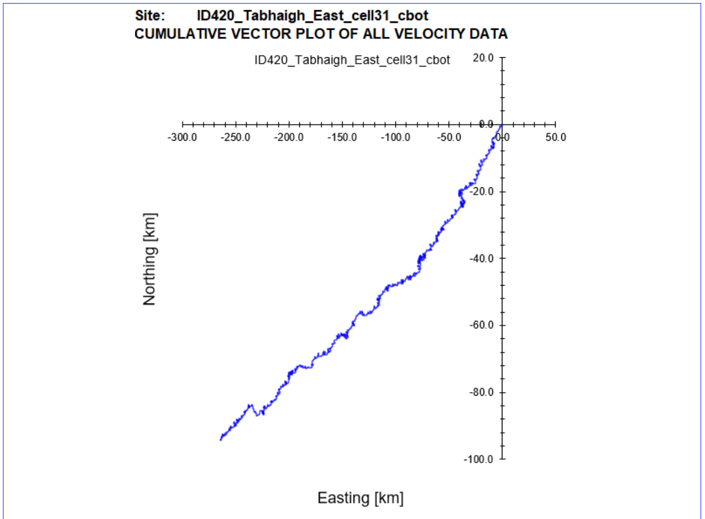
Figure 7. Cumulative Vector Plot of all velocity data from cage bottom cell for ID420.
