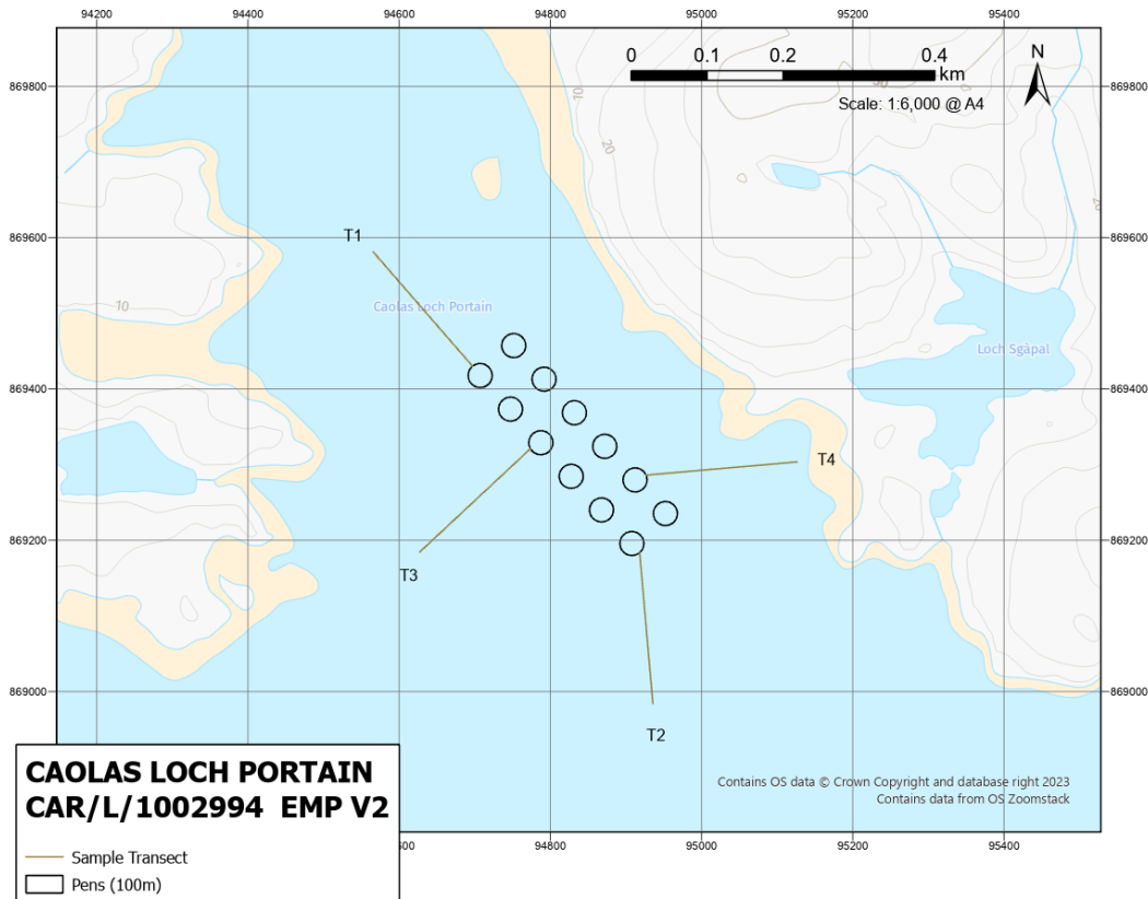
Figure 1 Plot illustrating the site location, layout, and proposed transects.
