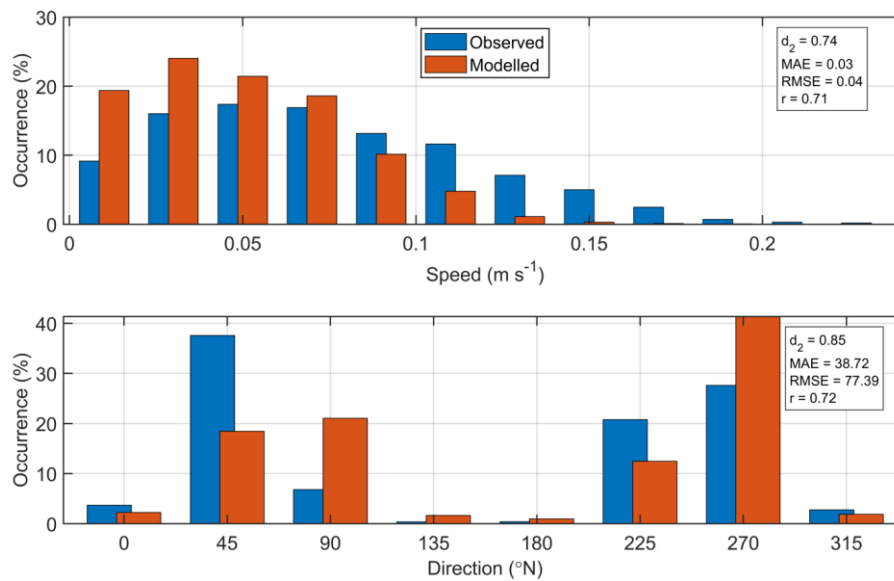
Figure 12. Histograms of observed and modelled current speed (top) and direction (bottom) at the ADCP location from May – July 2018 (ID218). Observed data are in blue, model results in red.
