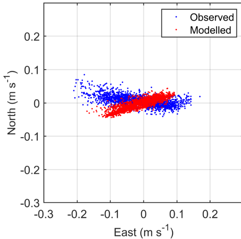
Figure 15. Scatter plot of observed and modelled velocity at the ADCP location from May – July 2018 (ID219). Observed data are in blue, model results in red.
