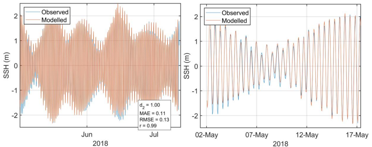
Figure 13. Comparison between observed and modelled sea surface height from May – July 2018 (ADCP deployment ID219) using model parameter values from Table 1. Both the full record (left) and a subset of 15 days (right) are shown. Observed data are in blue, model results in red.
