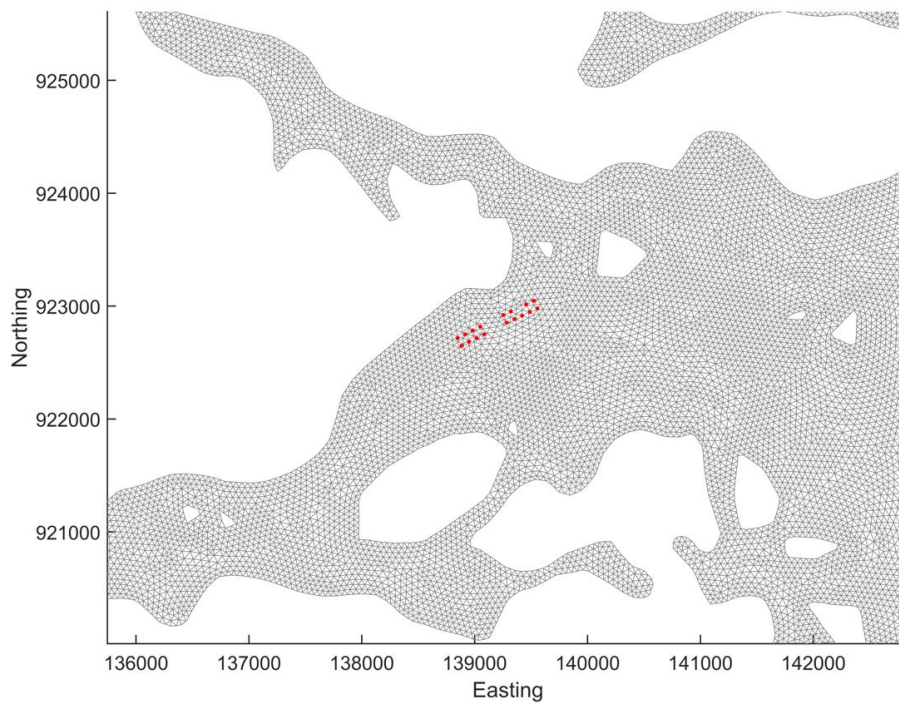
Figure 2. The unstructured mesh around the North Shore sites in the modified model grid, with the proposed cage locations indicated (•).
