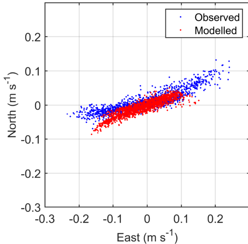
Figure 7. Scatter plot of observed and modelled velocity at the ADCP location from February – May 2018 (ID194). Observed data are in blue, model results in red.
