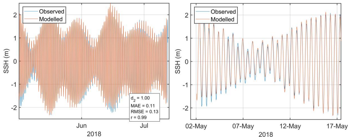
Figure 9. Comparison between observed and modelled sea surface height from May – July 2018 (ADCP deployment ID218) using model parameter values from Table 1. Both the full record (left) and a subset of 15 days (right) are shown. Observed data are in blue, model results in red.
