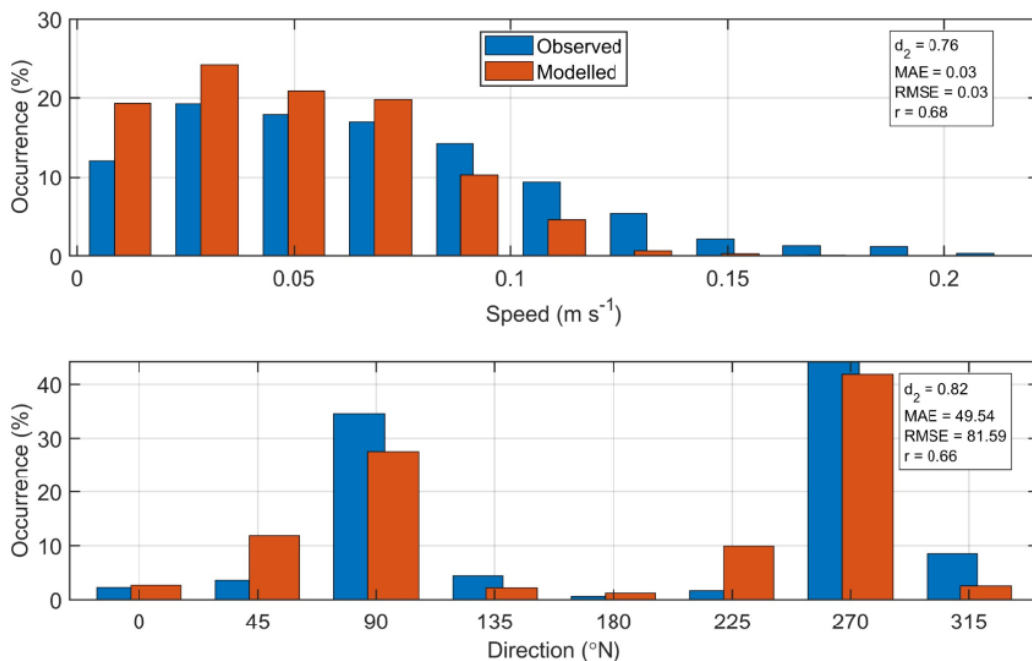
Figure 16. Histograms of observed and modelled current speed (top) and direction (bottom) at the ADCP location from May – July 2018 (ID219). Observed data are in blue, model results in red.
