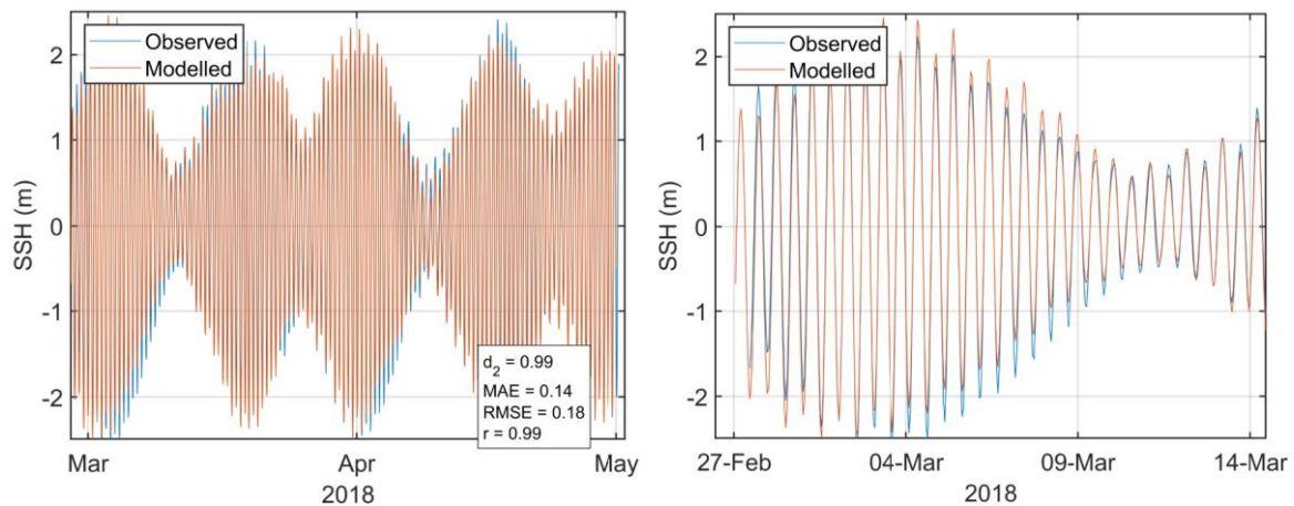
Figure 5. Comparison between observed and modelled sea surface height from February – May 2018 (ADCP deployment ID194) using model parameter values from Table 1. Both the full record (left) and a subset of 15 days (right) are shown. Observed data are in blue, model results in red.
