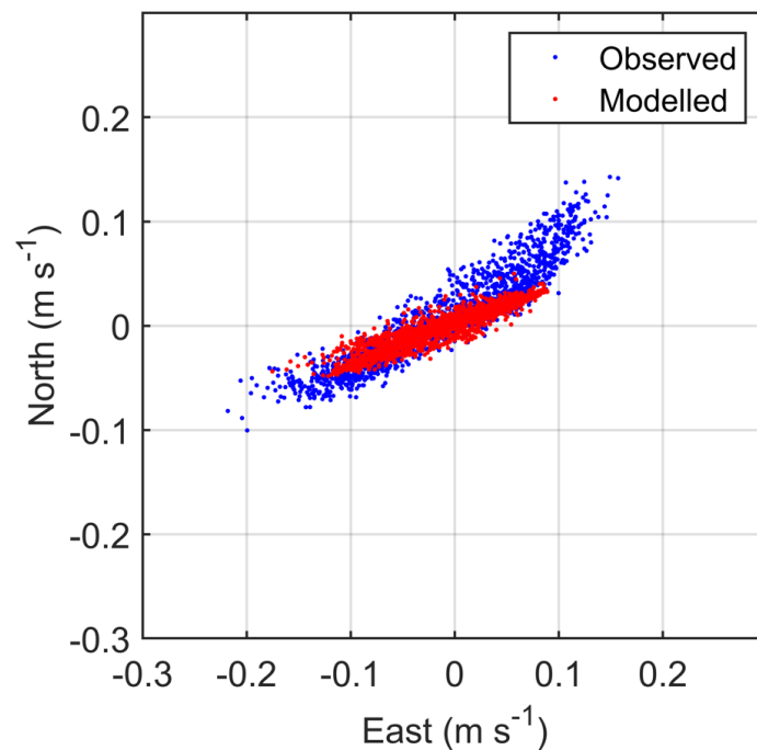
Figure 11. Scatter plot of observed and modelled velocity at the ADCP location from May – July 2018 (ID218). Observed data are in blue, model results in red.
