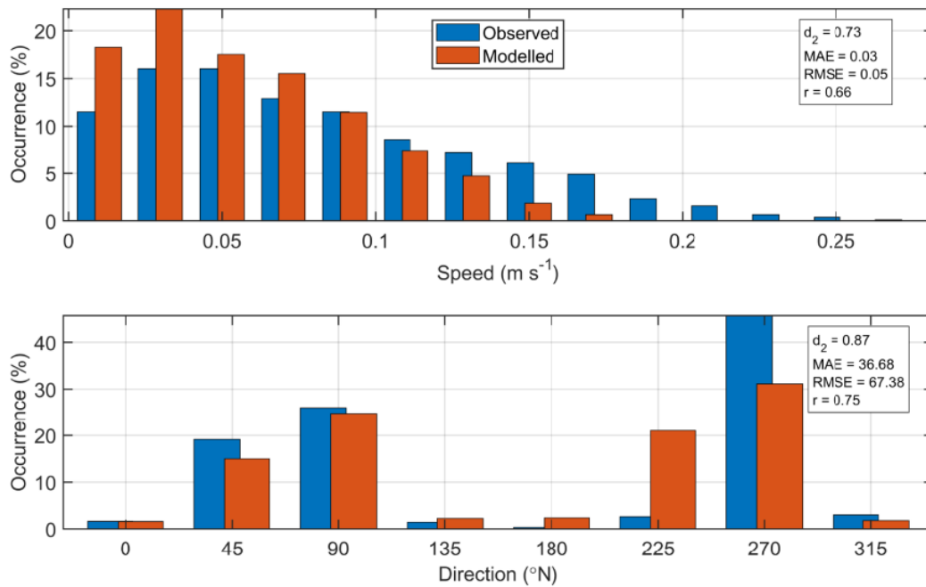
Figure 8. Histograms of observed and modelled speed (top) and direction (bottom) at the ADCP location from February – May 2018 (ID194). Observed data are in blue, model results in red.
