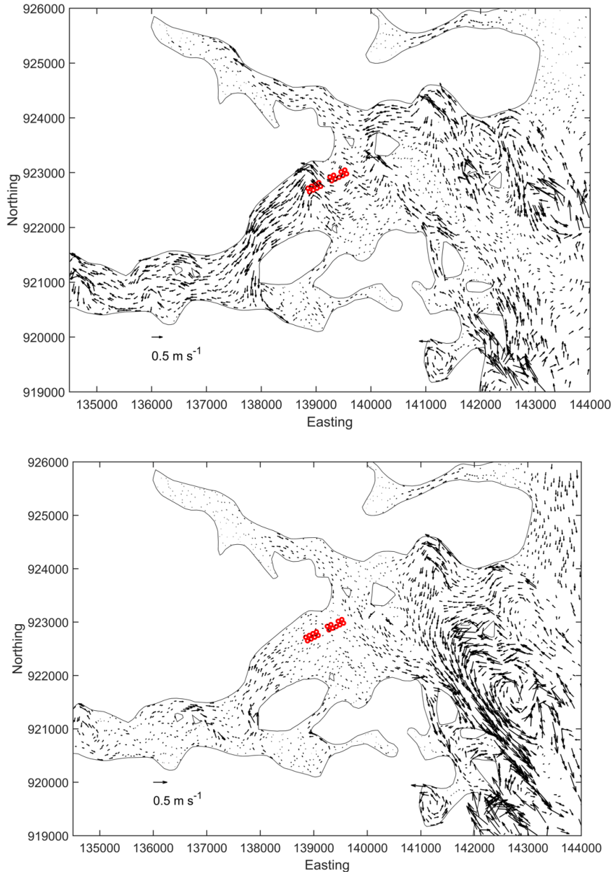
Figure 17. Modelled flood (top) and ebb (bottom) surface current vectors during spring tides. For clarity, only every 10 th vector is shown.
