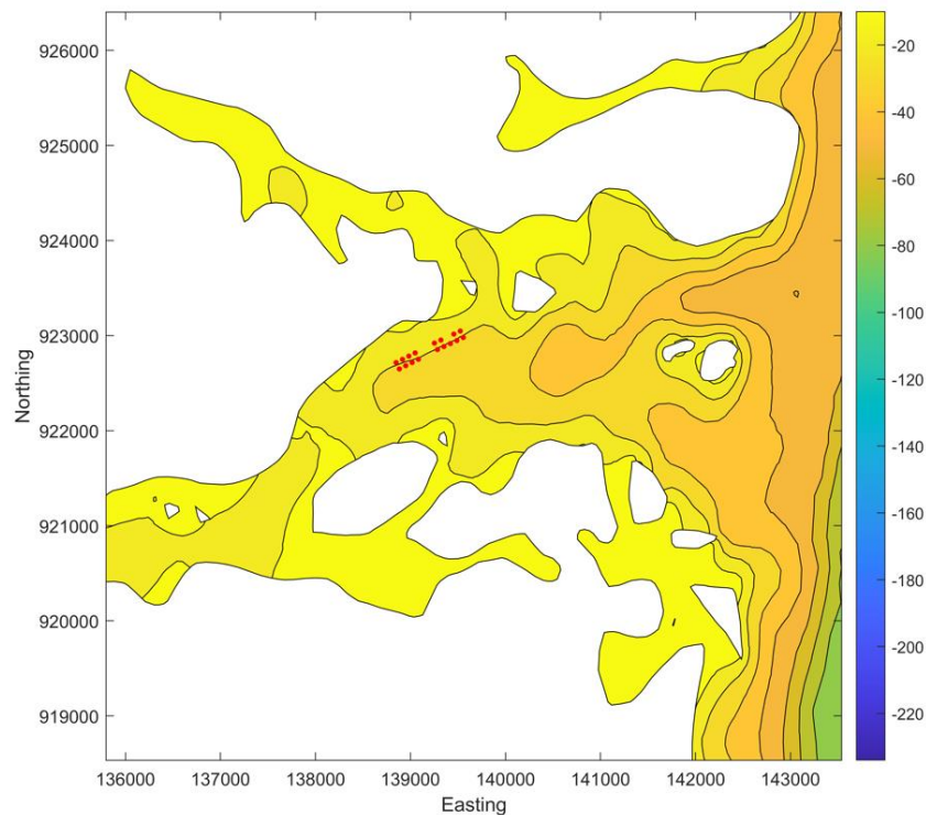
Figure 3. Model water depths (m) in the area around the North Shore salmon farms. The pen locations indicated (●).
