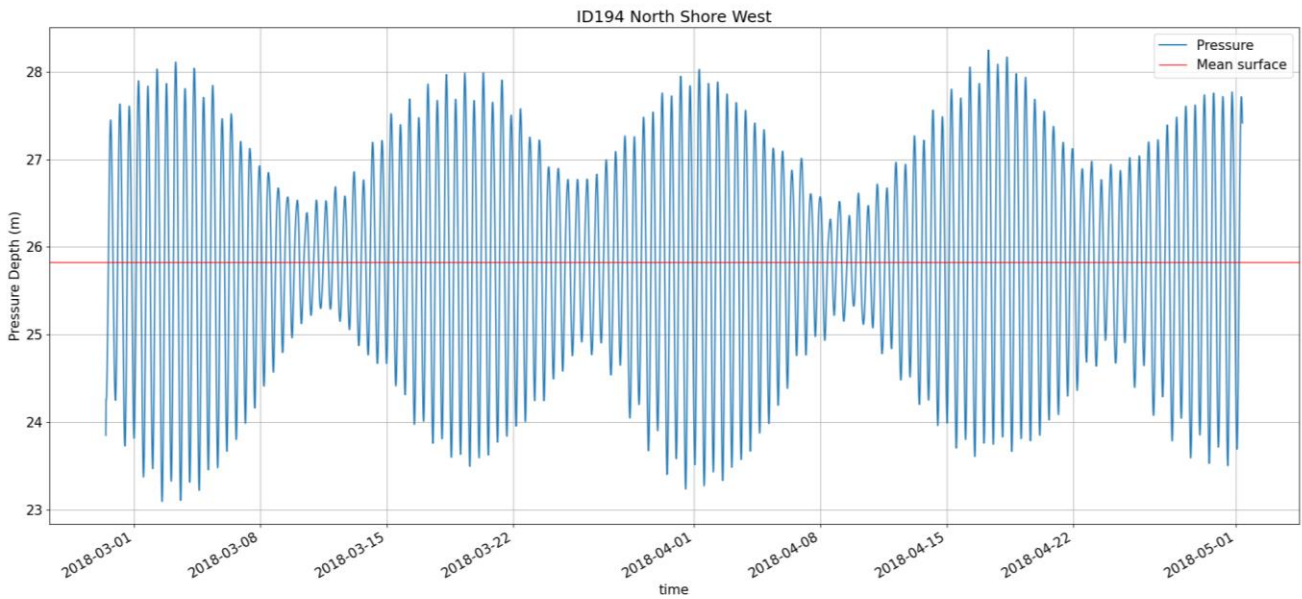
Figure 12. Pressure data from deployment ID194.
