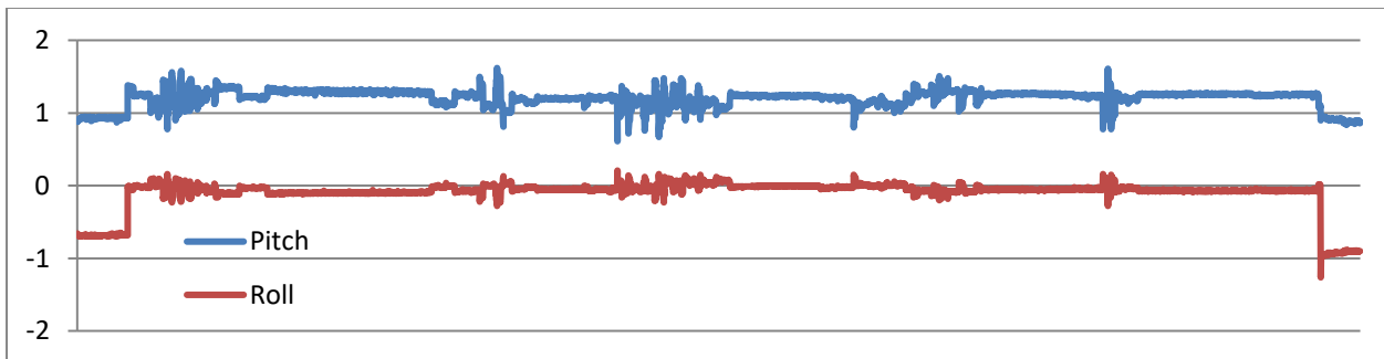
Figure 11. Summary of pitch and roll data from deployment ID280.
