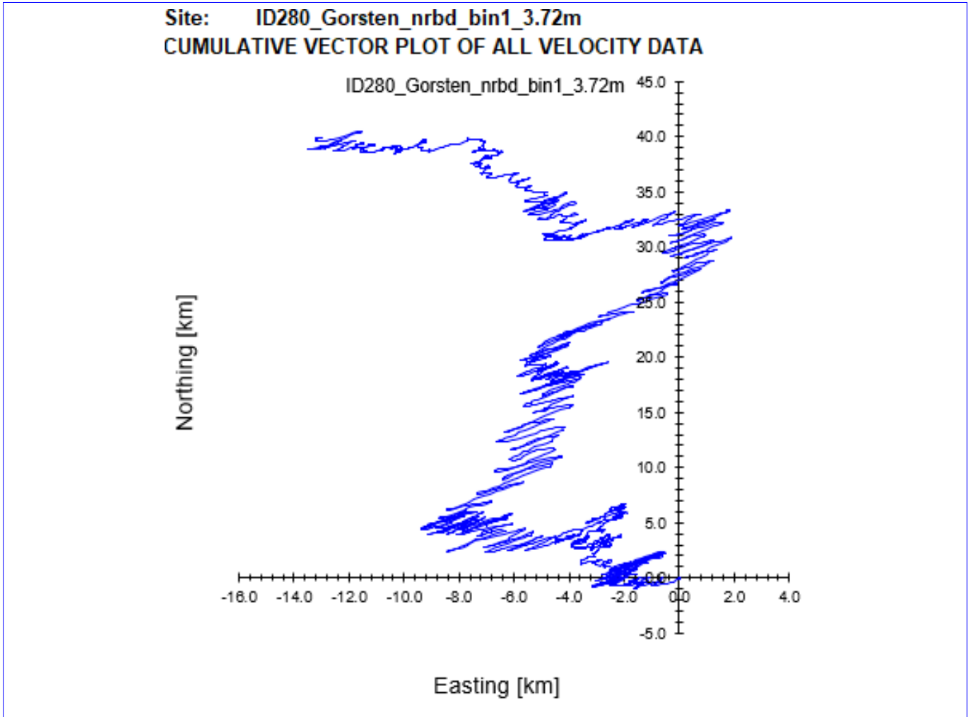
Figure 9. Cumulative Vector Plot of all velocity data from near bottom cell for ID280.
