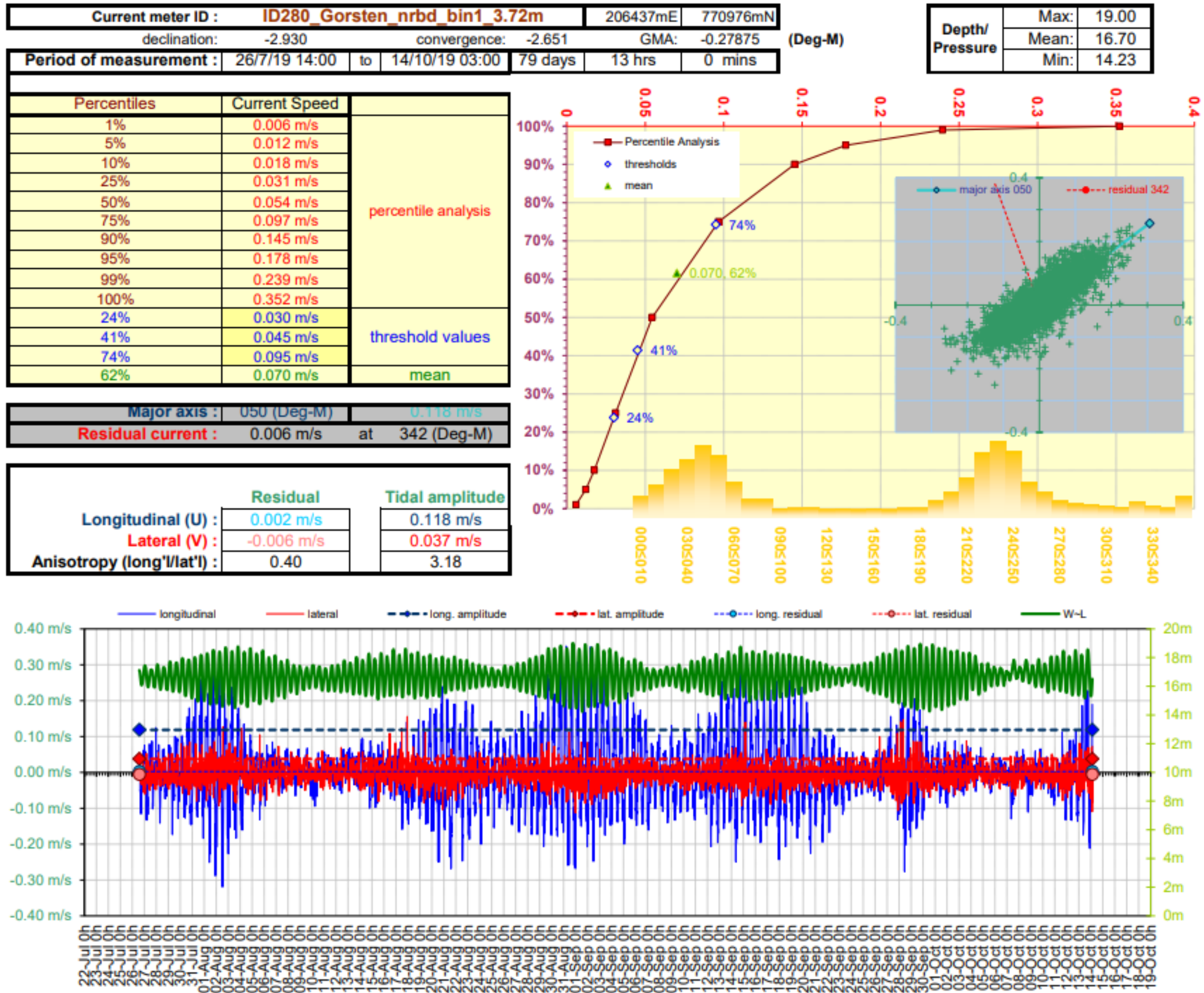
Figure 6. Current Data Summary Sheet for the near bottom current cell 1, 3.72m from seabed, 26 th July to 14 th October 2019 inclusive (ID280).
