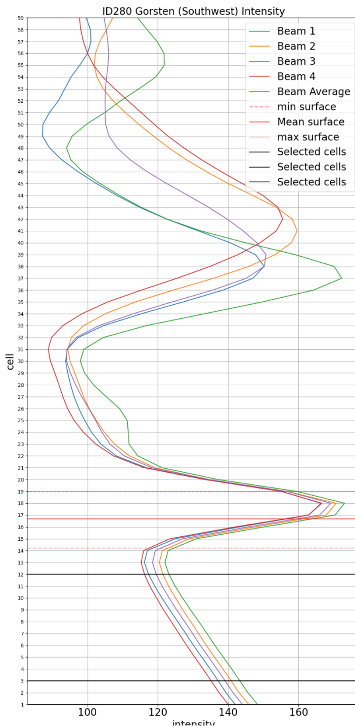
Figure 3. Mean intensity of the ADCP signal for the ID280 dataset plotted by bin number
