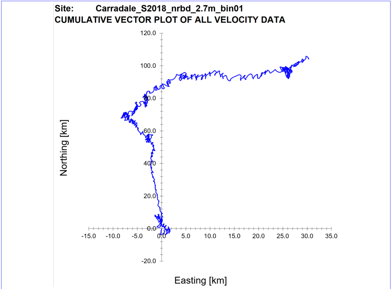
Figure 9. Cumulative Vector Plot of all velocity data from near bottom cell for ID119.
