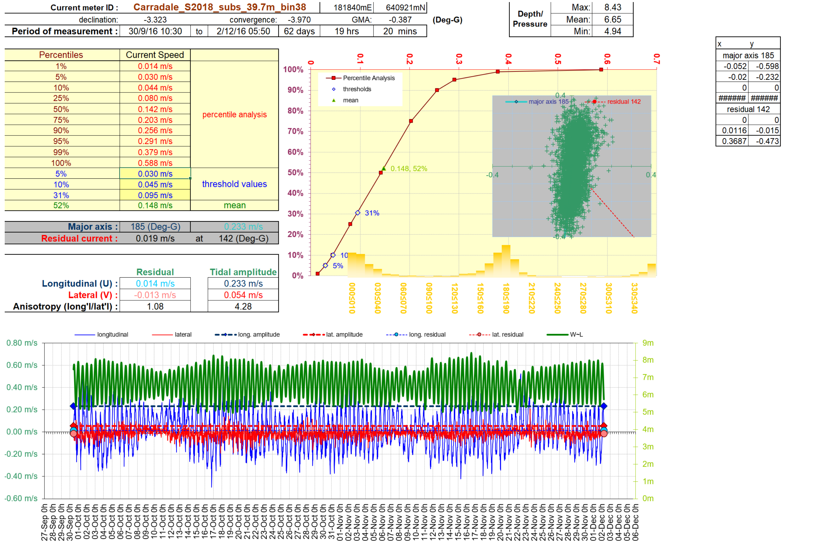
Figure 4. Current Data Summary Sheet for the surface current cell 38, 39.72m from seabed, 30 th September to 2 nd December 2016 inclusive (ID119).
