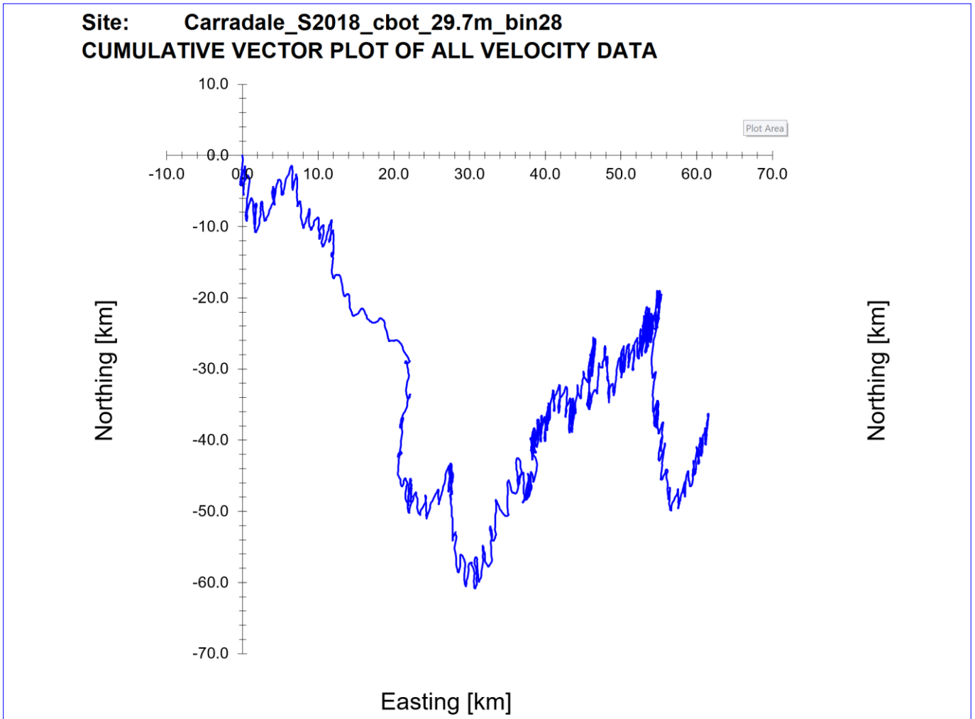
Figure 8. Cumulative Vector Plot of all velocity data from cage bottom cell for ID119.
