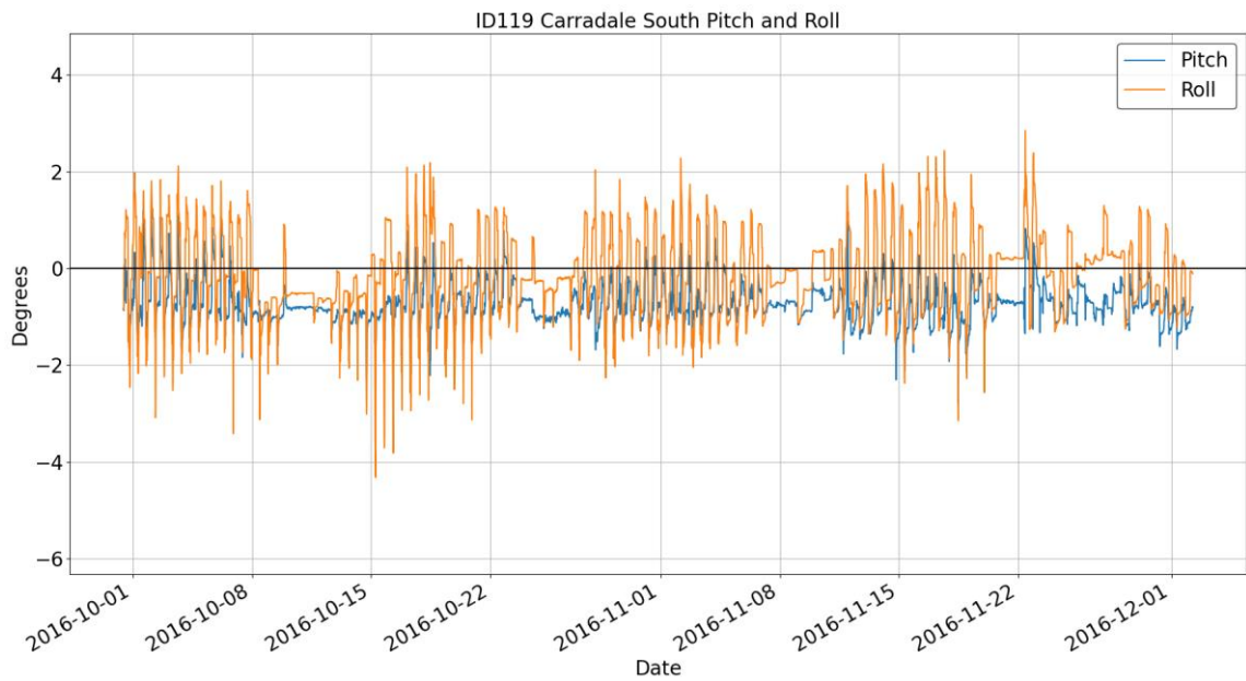
Figure 11. Summary of pitch and roll data from deployment ID119.
