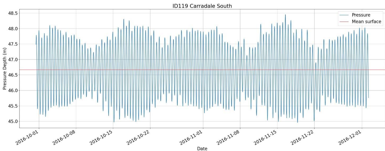
Figure 12. Pressure data from deployment ID119.
