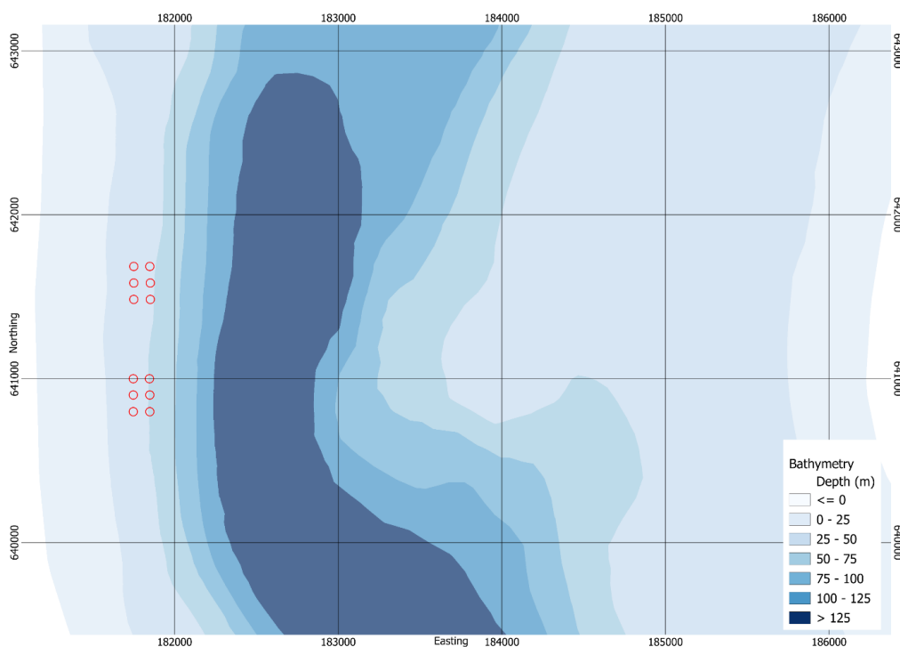
Figure 2. Bathymetry in Kilbrannan Sound, near the Carradale sites.
