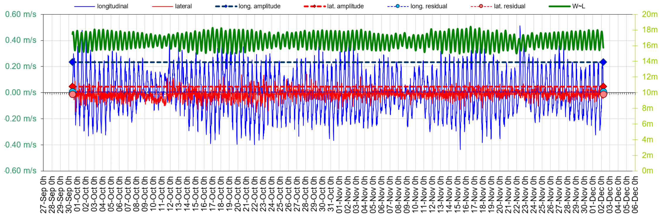
Figure 5. Current Data Summary Sheet for the cage bottom current cell 28, 29.72m from seabed, 30 th September to 2 nd December 2016 inclusive (ID119).
