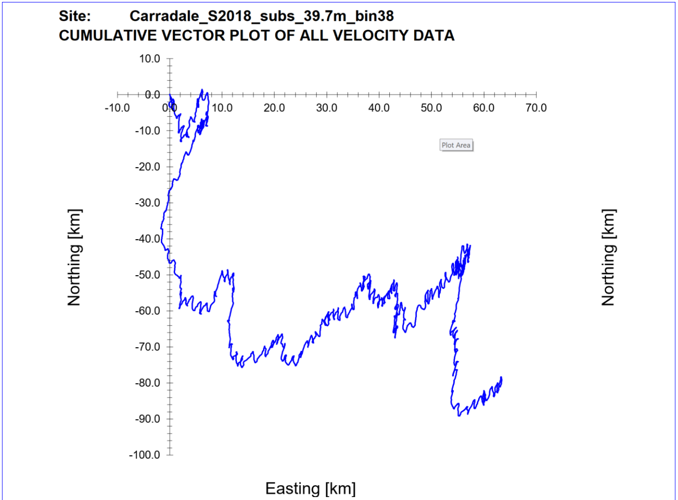
Figure 7. Cumulative Vector Plot of all velocity data from near surface cell for ID119.
