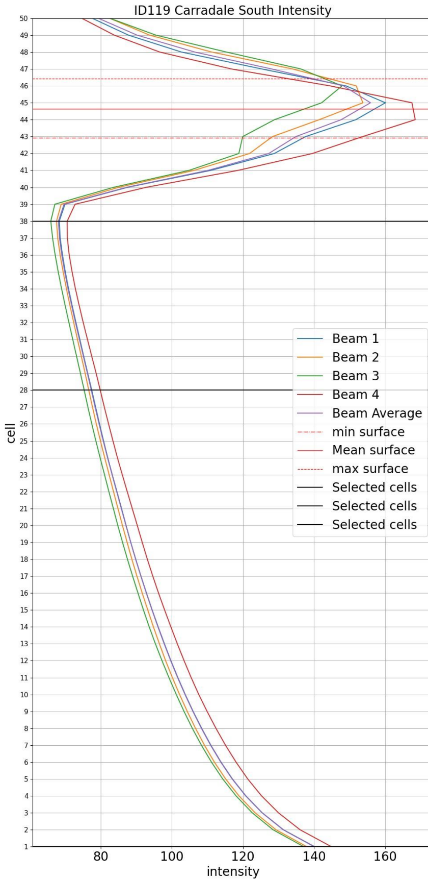
Figure 3. Mean intensity of the ADCP signal for the ID119 dataset plotted by bin number
