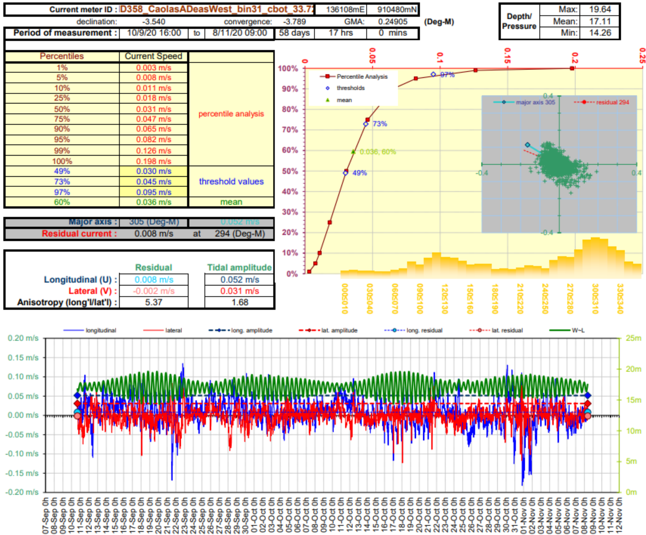
Figure 5. Current Data Summary Sheet for the cage bottom current cell 31, 33.72m from seabed, 10 th September to 8 th November 2020 inclusive (ID358).
