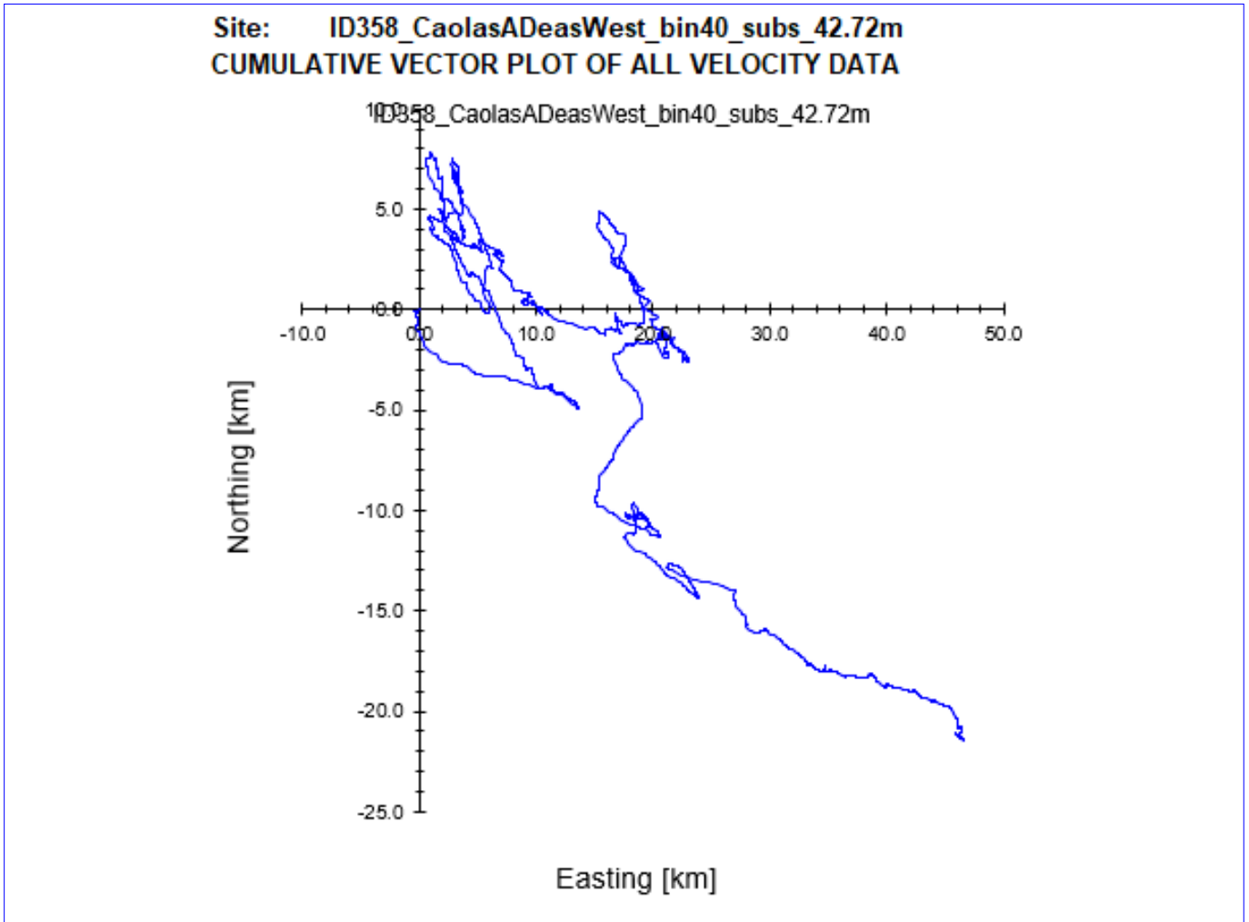
Figure 7. Cumulative Vector Plot of all velocity data from near surface cell for ID358.
