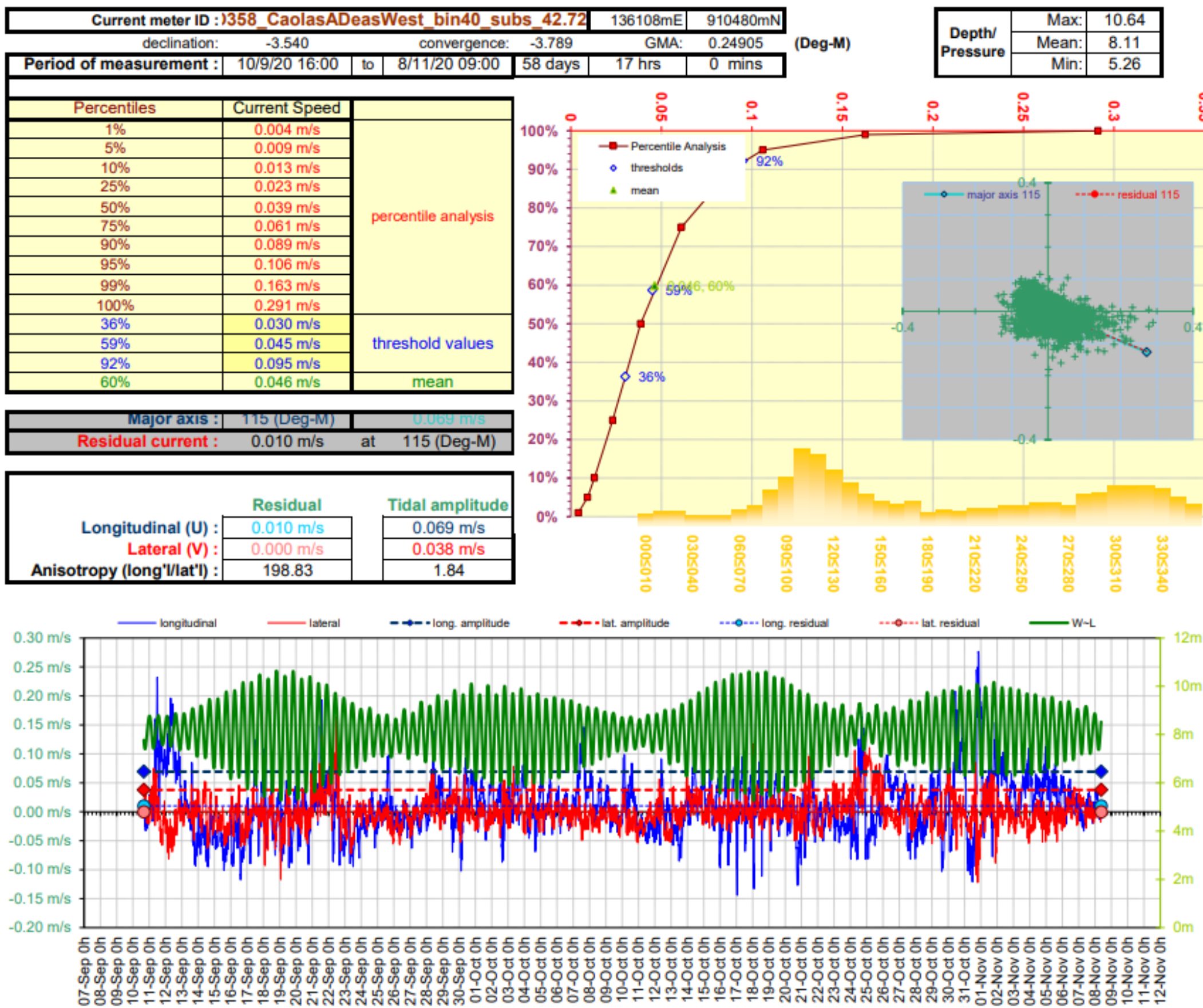
Figure 4. Current Data Summary Sheet for the surface current cell 40, 42.72m from seabed, 10 th September to 8 th November 2020 inclusive (ID358).
