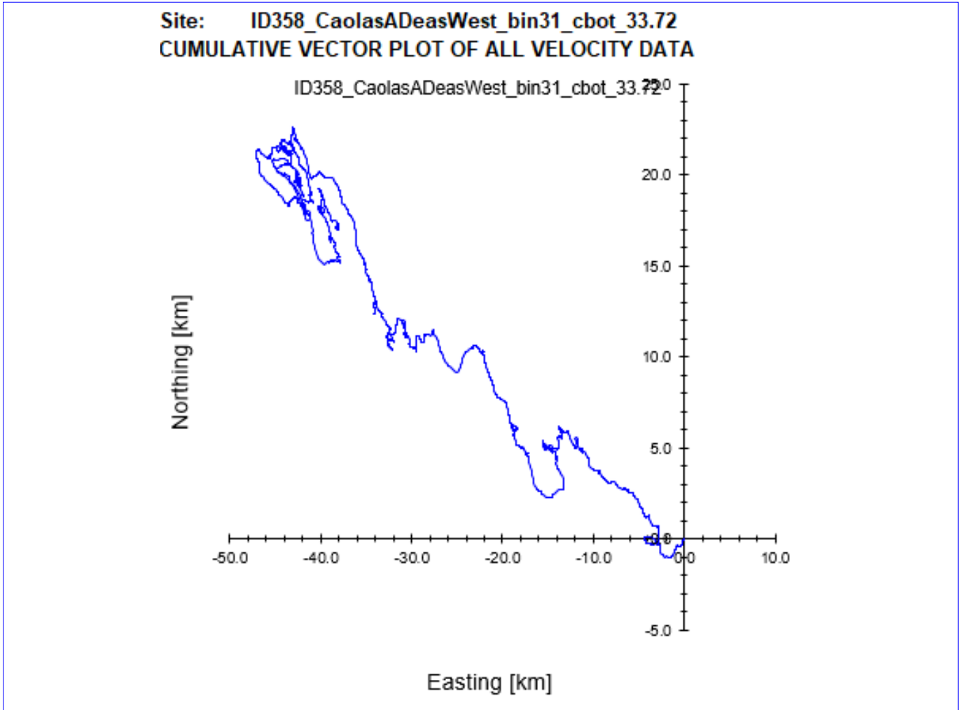
Figure 8. Cumulative Vector Plot of all velocity data from cage bottom cell for ID358.
