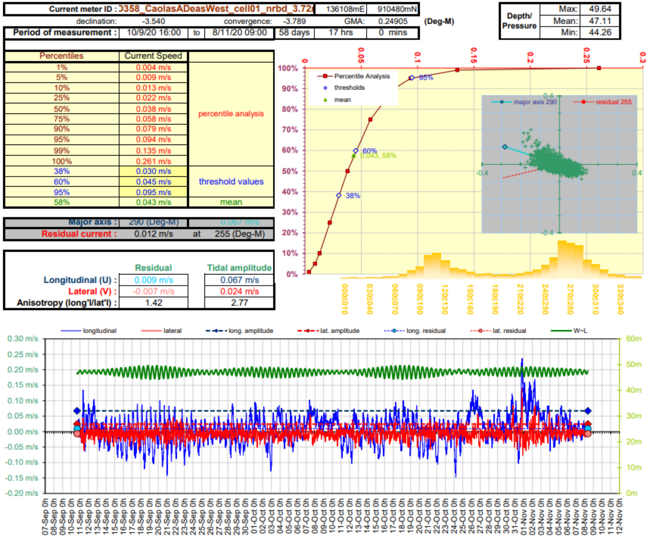
Figure 6. Current Data Summary Sheet for the near bottom current cell 1, 3.7m from seabed, 10 th September to 8 th November 2020 inclusive (ID358).
