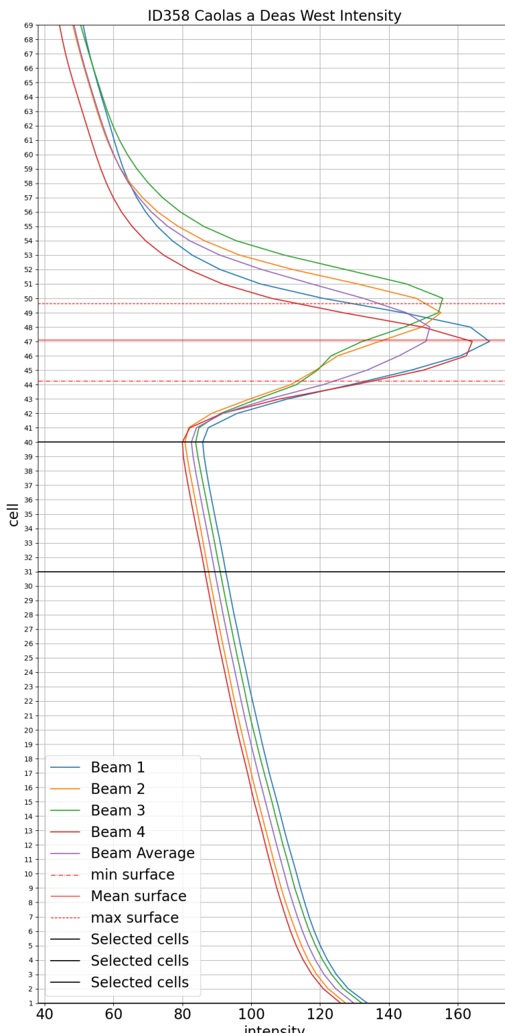
Figure 3. Mean intensity of the ADCP signal for the ID358 dataset plotted by bin number
