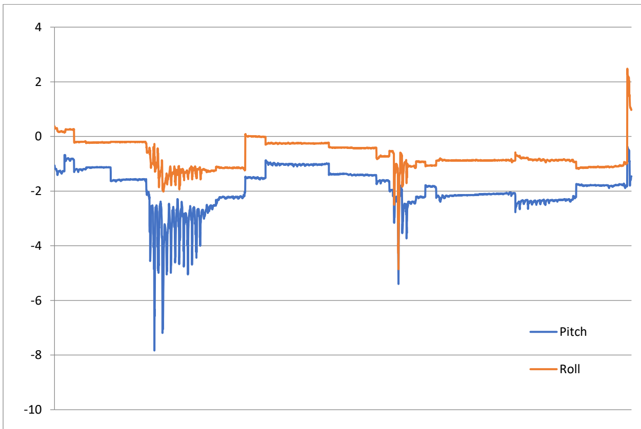
Figure 11. Summary of pitch and roll data from deployment ID218.
