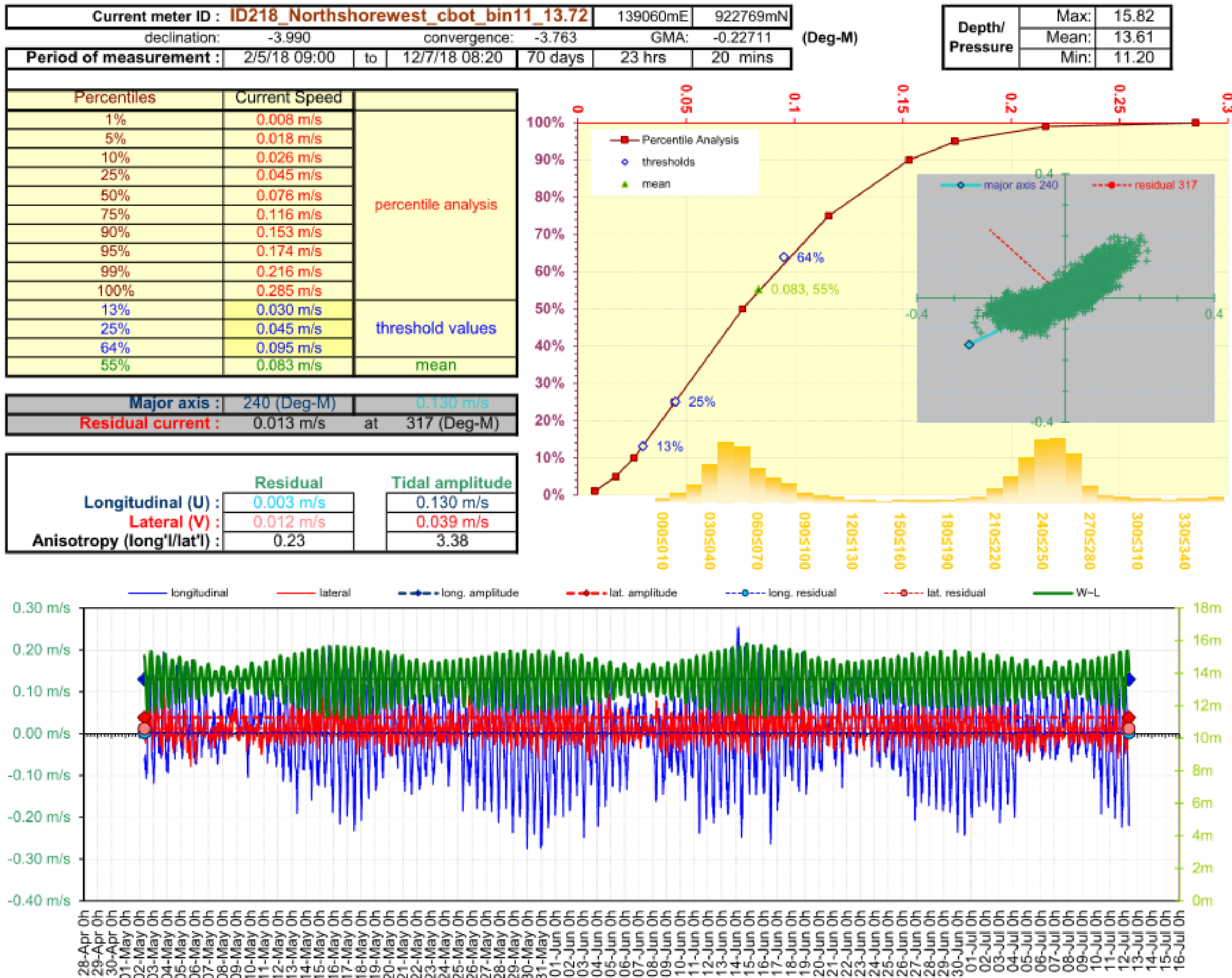
Figure 5. Current Data Summary Sheet for the cage bottom current cell 11, 13.72 m from seabed, 2 nd May to 12 th July 2018 inclusive (ID218).
