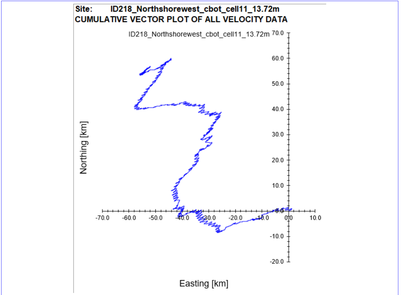
Figure 8. Cumulative Vector Plot of all velocity data from cage bottom cell for ID218.
