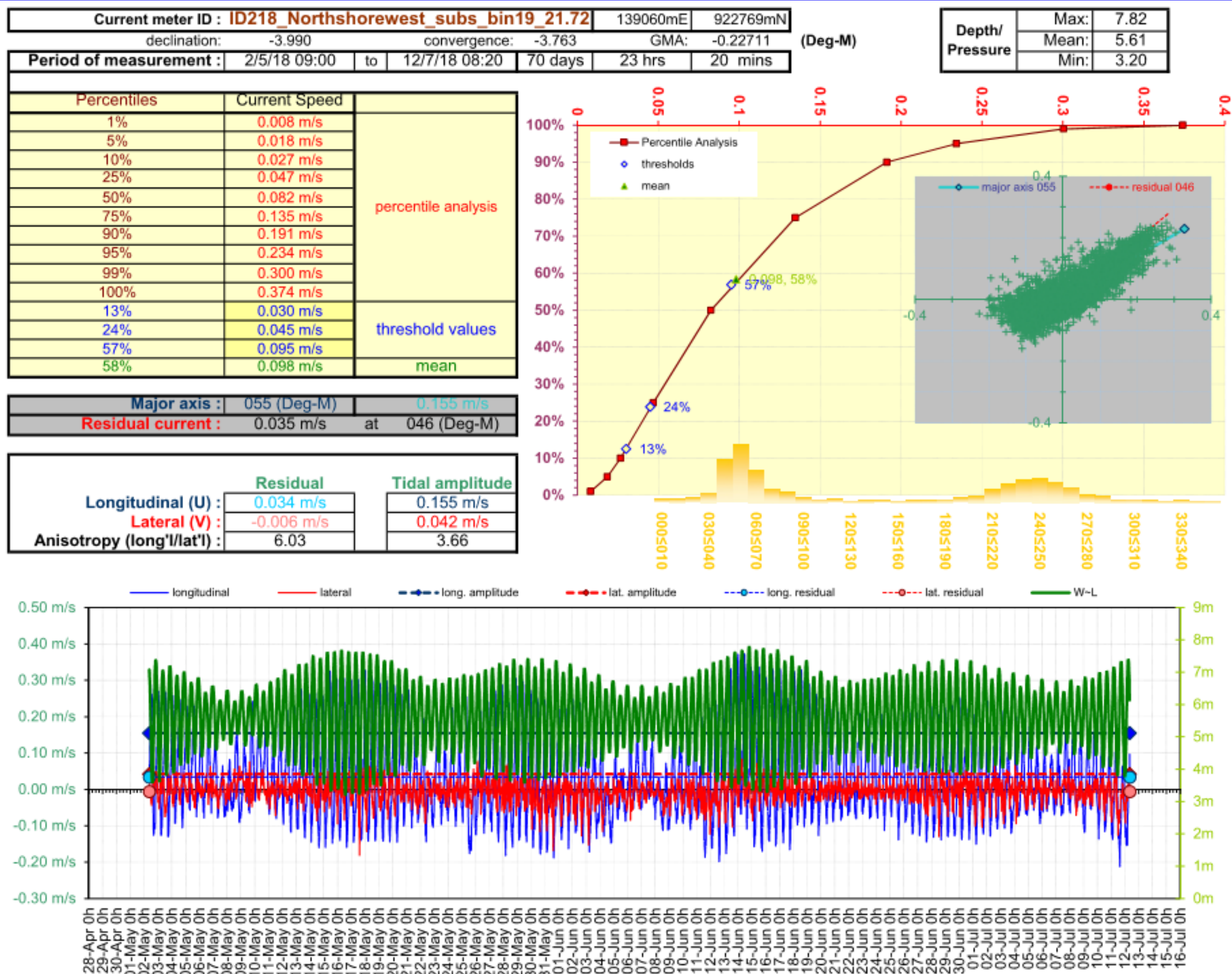
Figure 4. Current Data Summary Sheet for the surface current cell 19, 21.72 m from seabed, 2 nd May to 12 th July 2018 inclusive (ID218).
