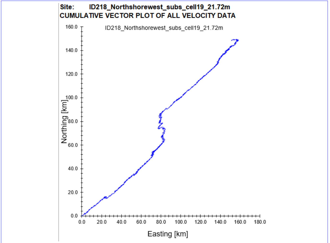
Figure 7. Cumulative Vector Plot of all velocity data from near surface cell for ID218.
