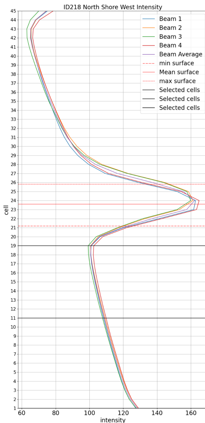
Figure 3. Mean intensity of the ADCP signal for the ID218 dataset plotted by bin number.
