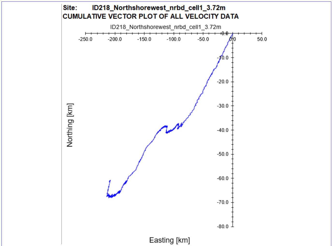
Figure 9. Cumulative Vector Plot of all velocity data from near bottom cell for ID218.
