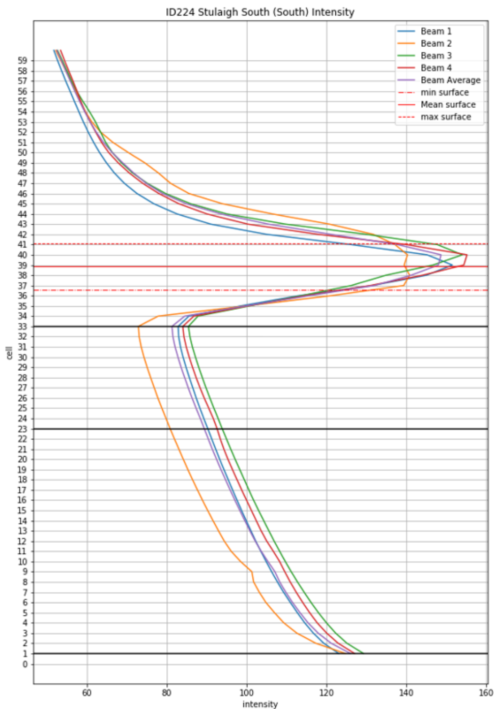
Figure 3. Mean intensity of the ADCP signal for the ID224 dataset plotted by bin number
