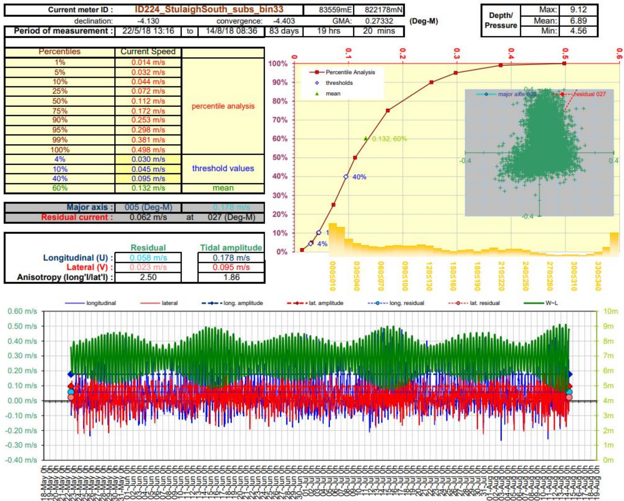
Figure 4. Current Data Summary Sheet for the surface current cell 33, 35.7m from seabed, 22 nd May to 14 th August 2018 inclusive (ID224).
