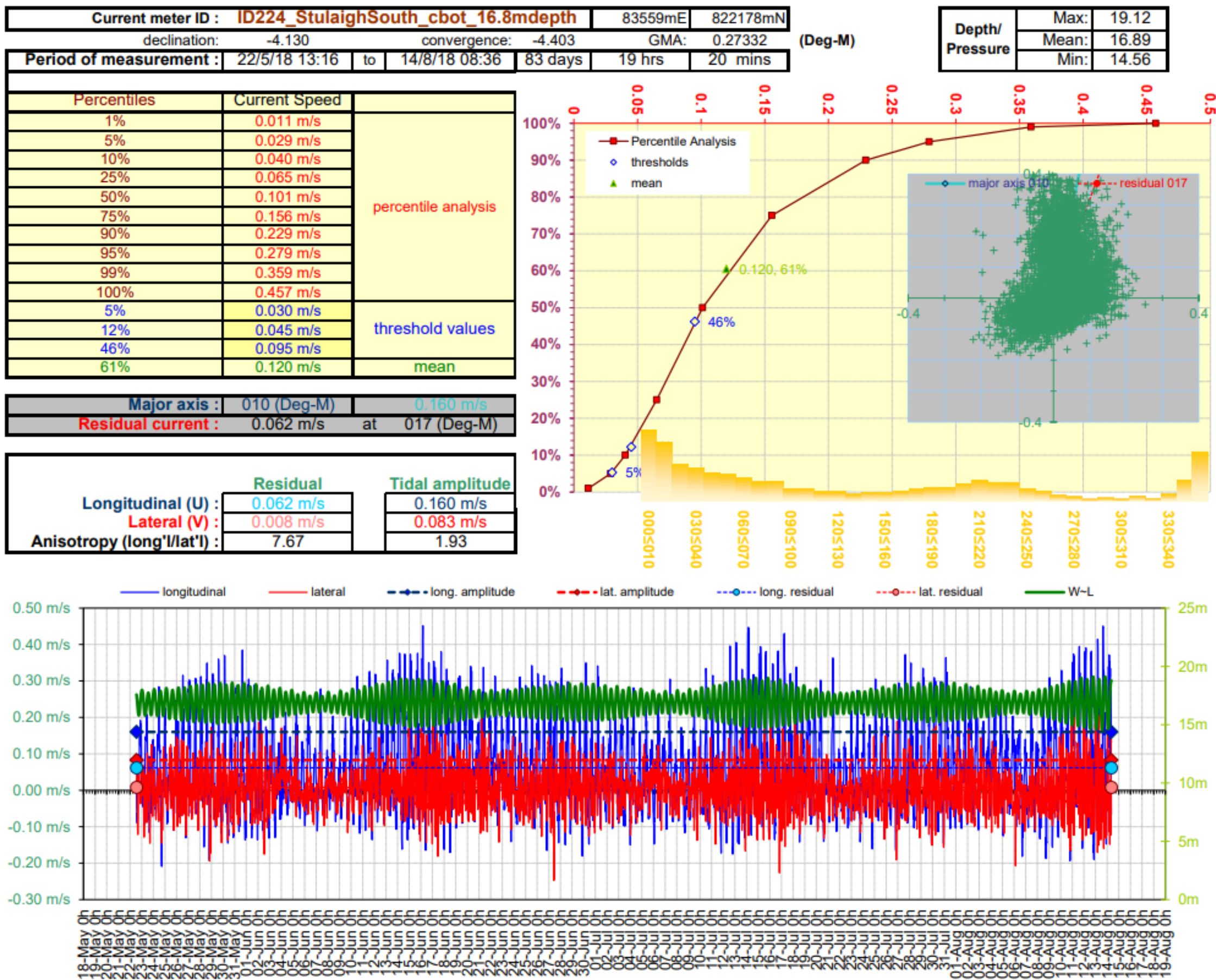
Figure 5. Current Data Summary Sheet for the cage bottom current cell 23, 25.7m from seabed, 22 nd May to 14 th August 2018 inclusive (ID224).
