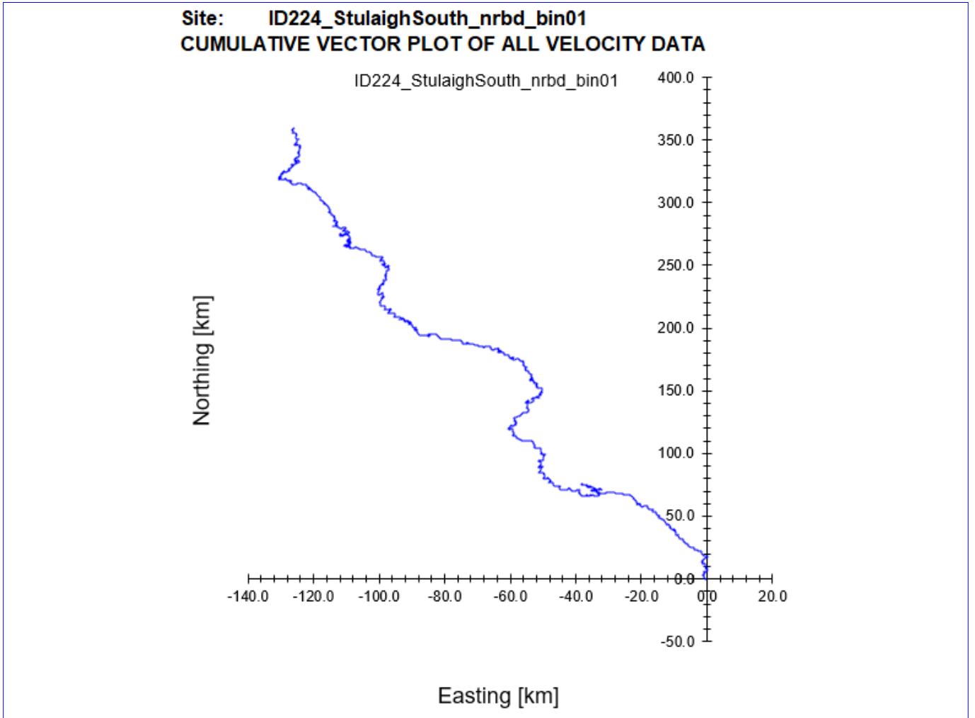
Figure 9. Cumulative Vector Plot of all velocity data from near bottom cell for ID224.
