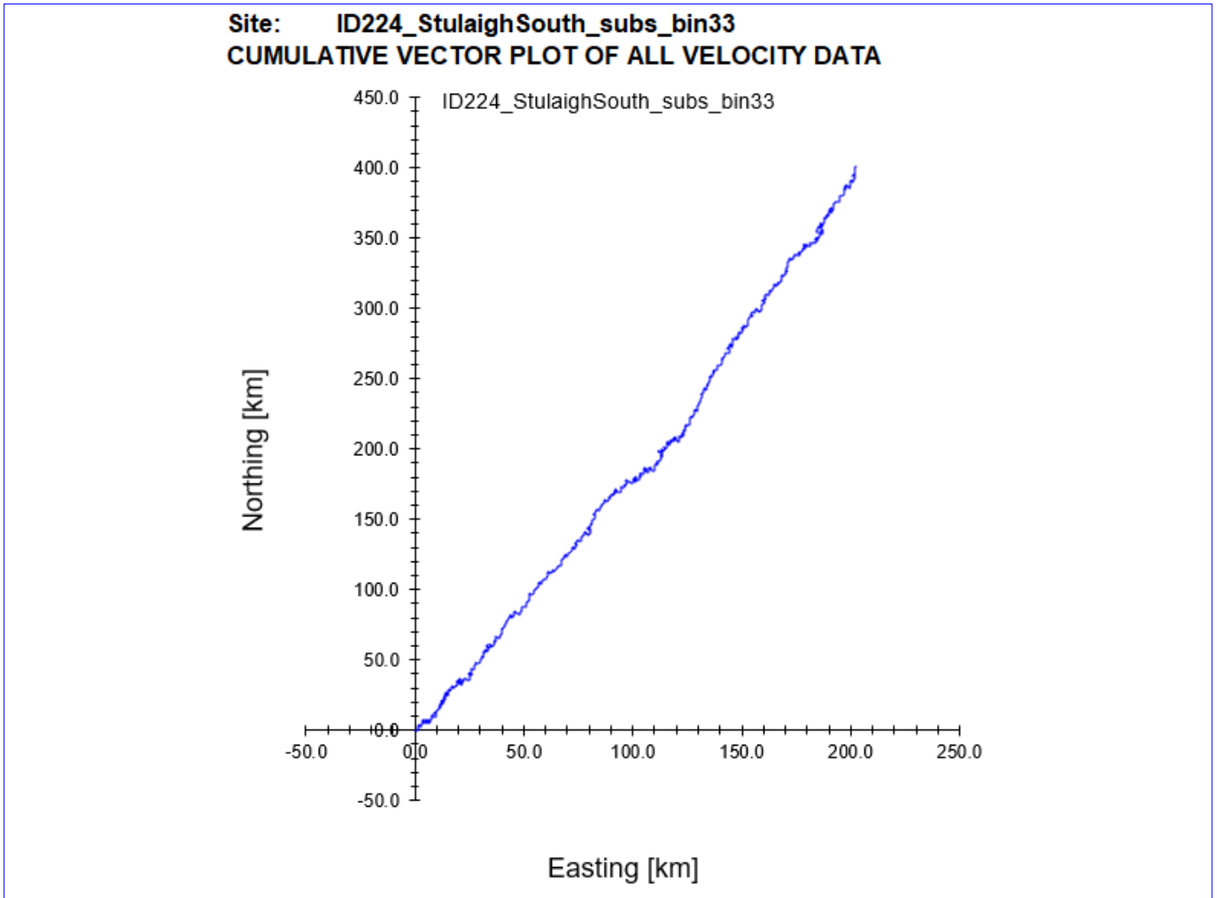
Figure 7. Cumulative Vector Plot of all velocity data from near surface cell for ID224.
