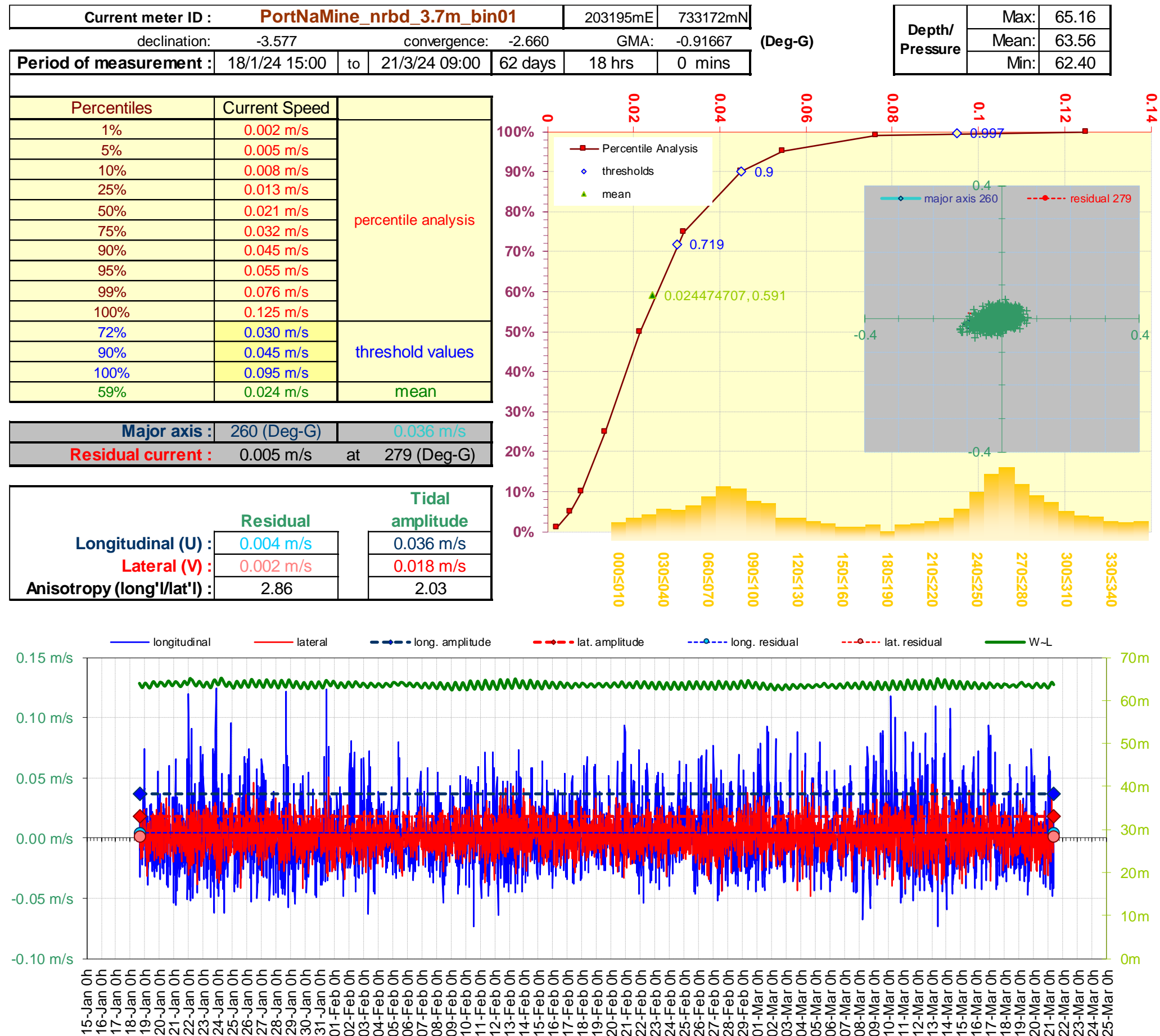
Figure 5. Current Data Summary Sheet for the near bottom current cell 1, 3.7m from seabed, 18 th January to 21 st March 2024 inclusive (ID434).
