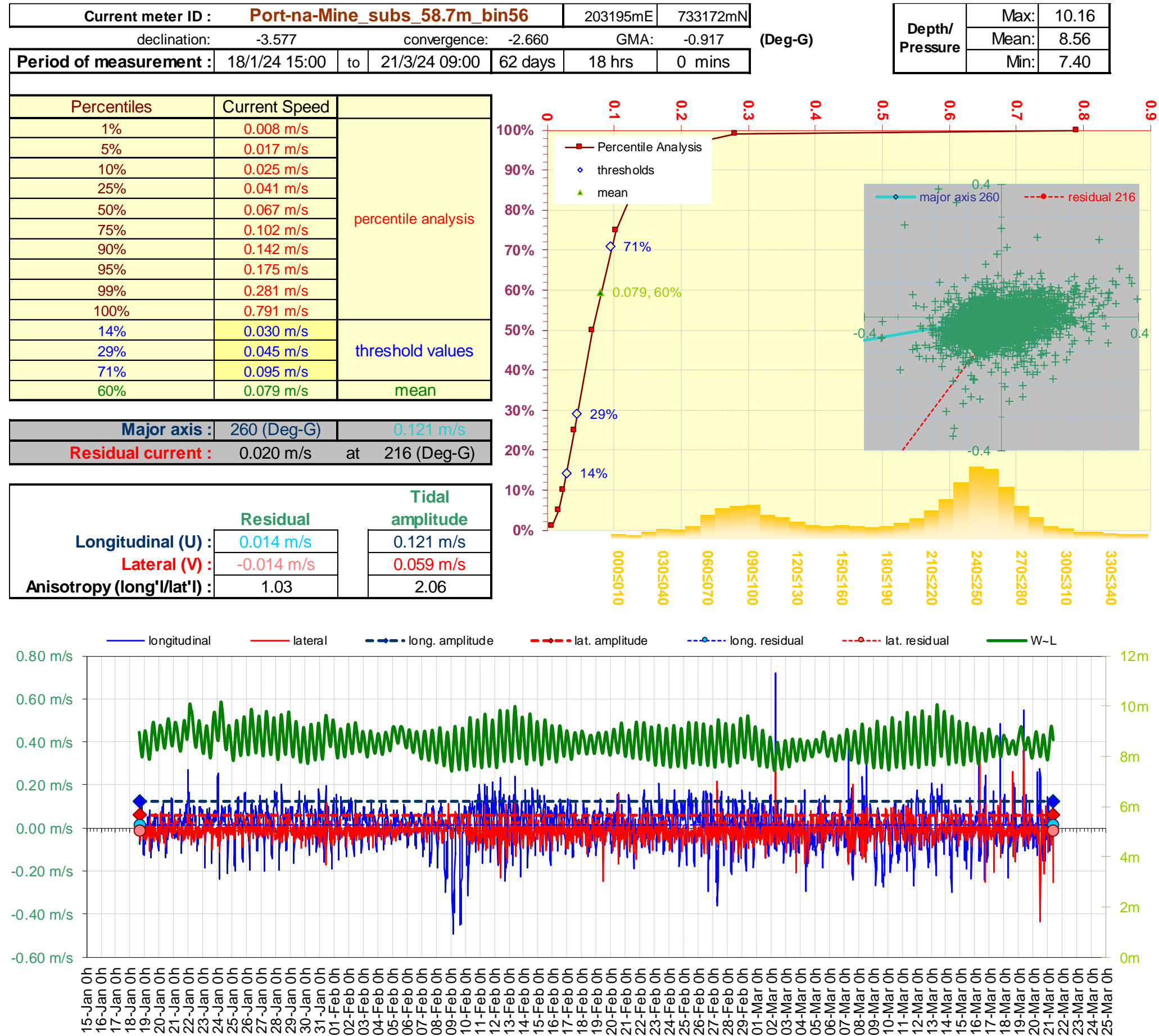
Figure 3. Current Data Summary Sheet for the surface current cell 56, 58.7m from seabed, 18 th January to 21 st March 2024 inclusive (ID434).
