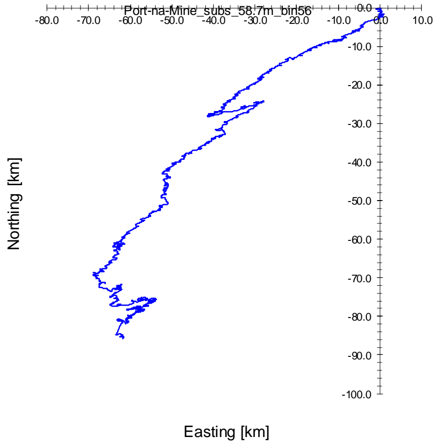
Figure 6. Cumulative Vector Plot of all velocity data from near surface cell for ID434.
