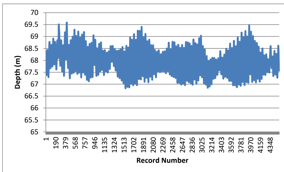
Figure 11. Pressure data from deployment ID434.
