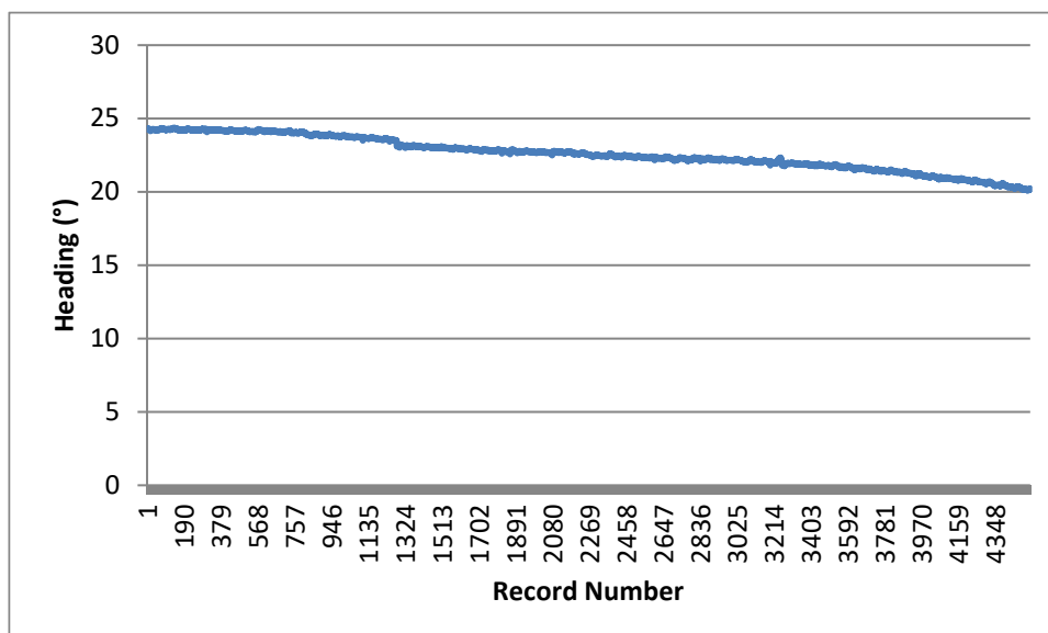
Figure 9. Summary of heading data from deployment ID434.
