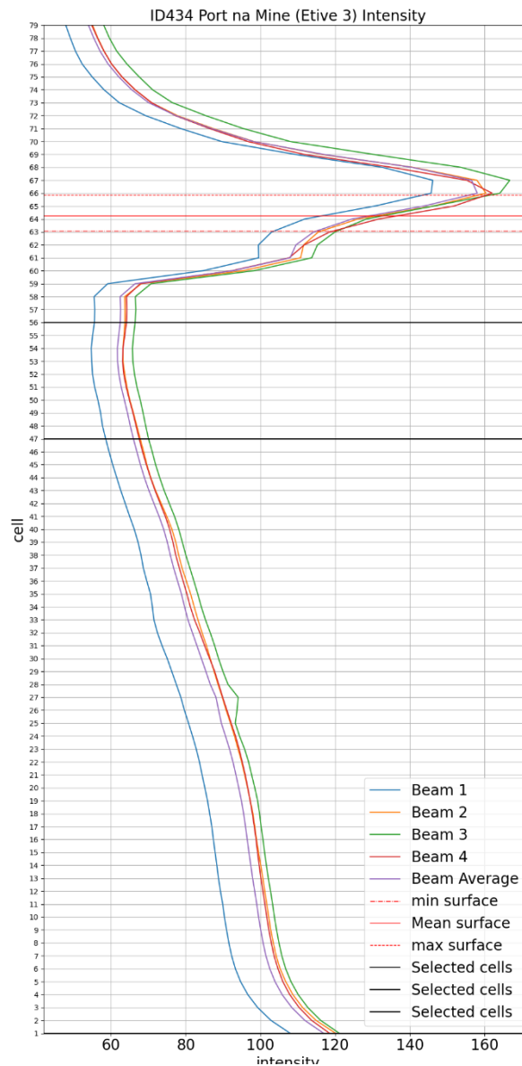
Figure 2. Mean intensity of the ADCP signal for the ID434 dataset plotted by bin number
