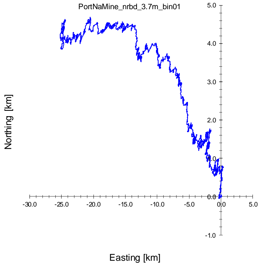
Figure 8. Cumulative Vector Plot of all velocity data from near bottom cell for ID434.
