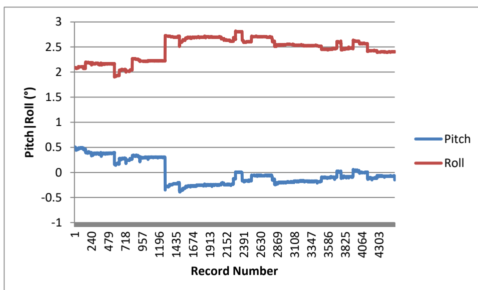
Figure 10. Summary of pitch and roll data from deployment ID434.
