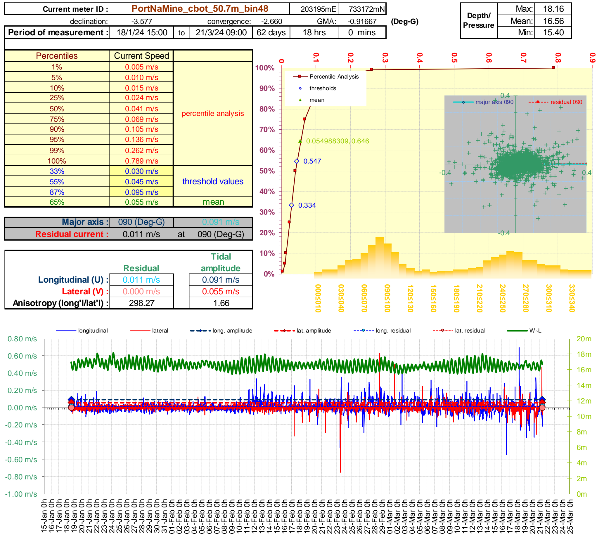
Figure 4. Current Data Summary Sheet for the cage bottom current cell 48, 50.7m from seabed, 18 th January to 21 st March 2024 inclusive (ID434).
