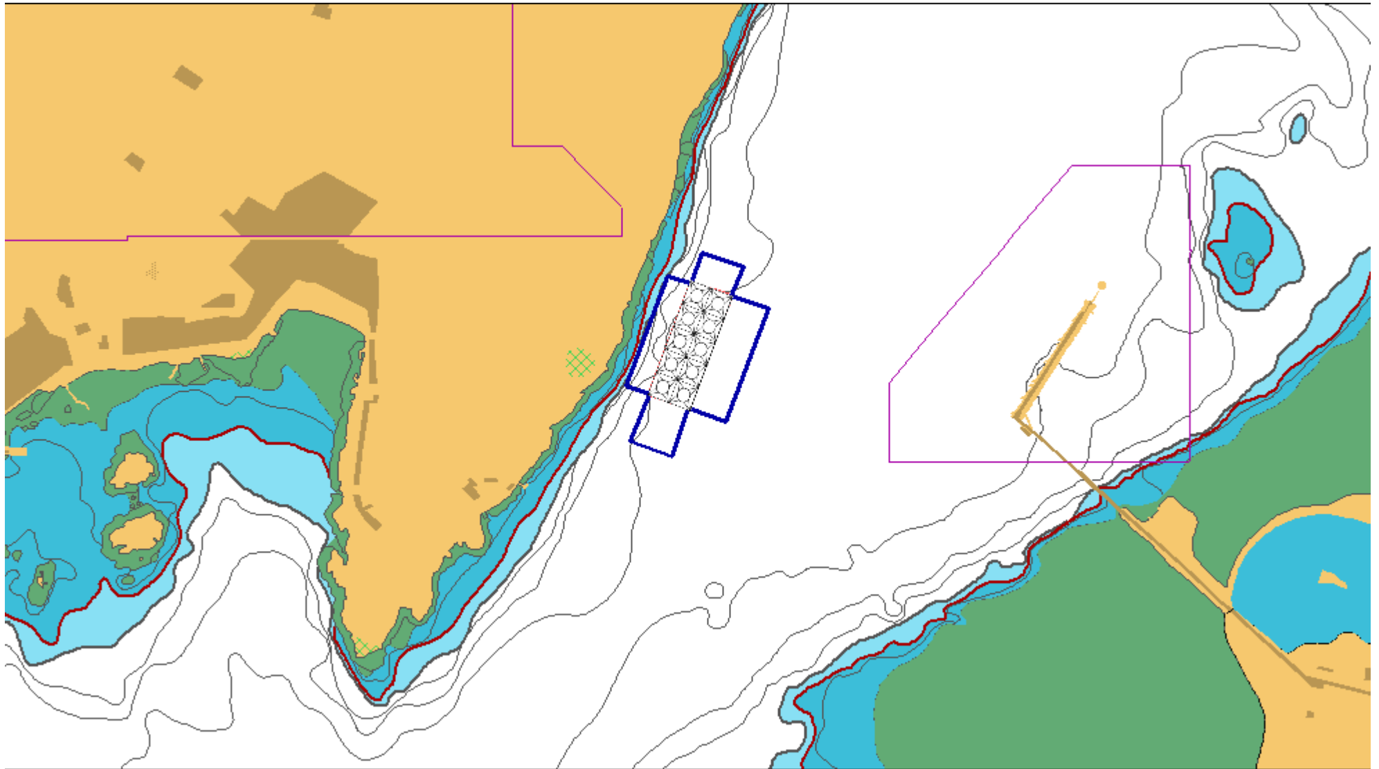
Figure 1: Proposed Cumrae Fish Farm Site, 5 x 2 configuration, 75m x 65m grid, 10 x 120m circumference pens.
