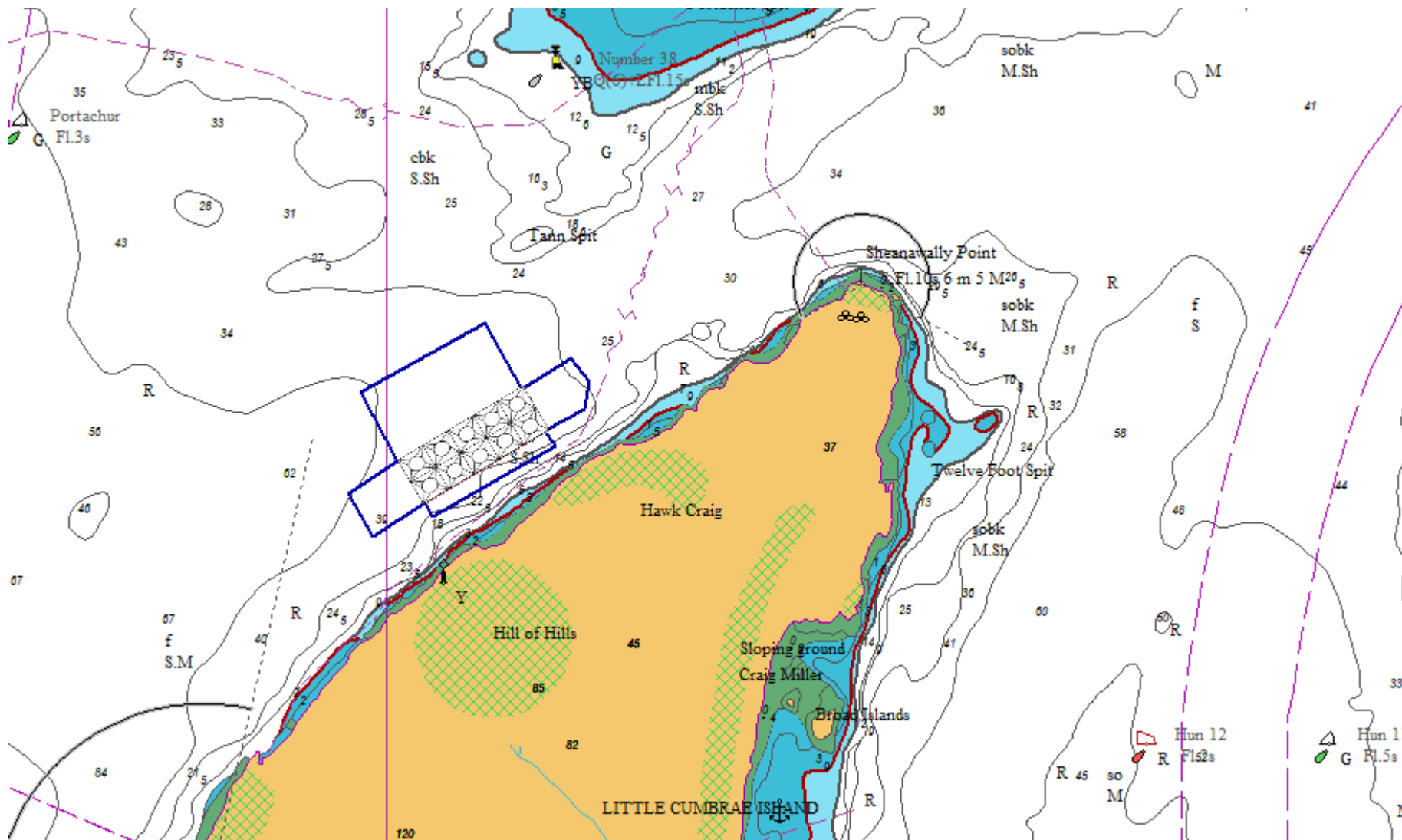
Figure 1: Proposed Little Cumbrae Fish Farm Site, 5 x 2 configuration, 80m x 75m grid, 10 x 120m circumference pens.
