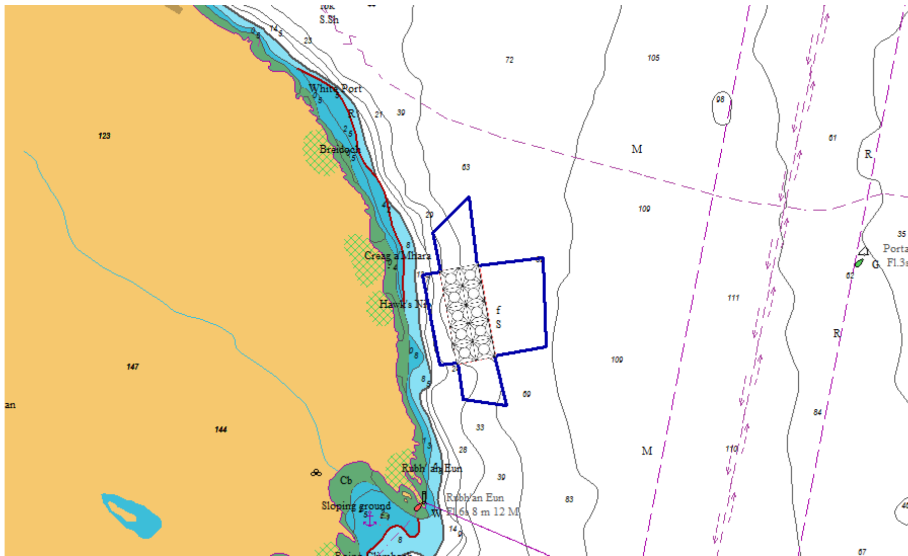
Figure 1: Proposed South Bute Fish Farm Site, 5 x 2 configuration, 75m grid, 10 x 120m circumference pens.
