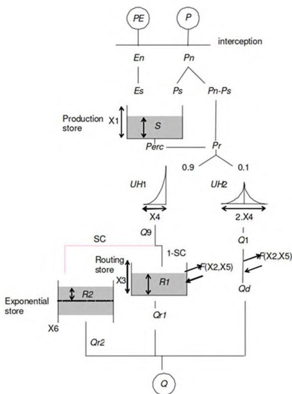
Figure B.1: GR6J model schematic
