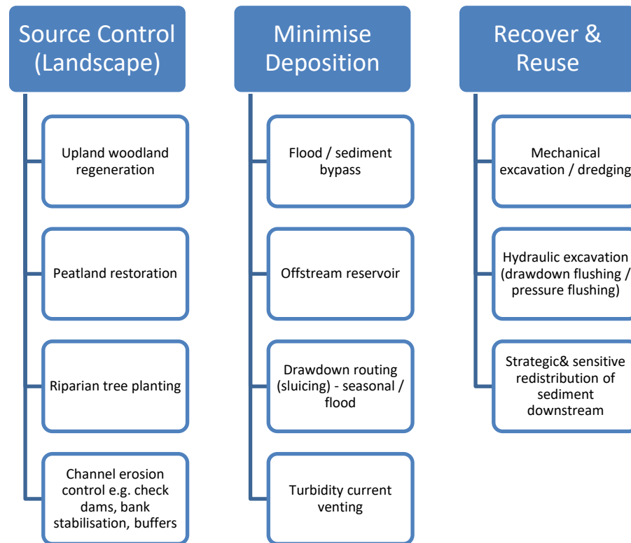
Figure 5-2: Indicative framework & example options for sediment management
