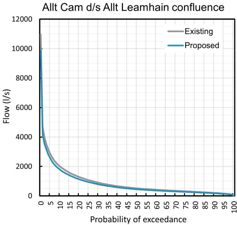
Figure 2.7: Existing and proposed flow duration curve – CA-PAT
