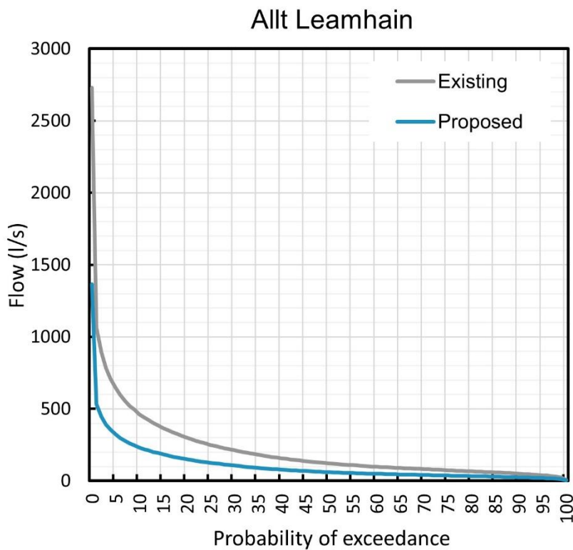
Figure 2.5: Existing and proposed flow duration curve – BH-BHE update
