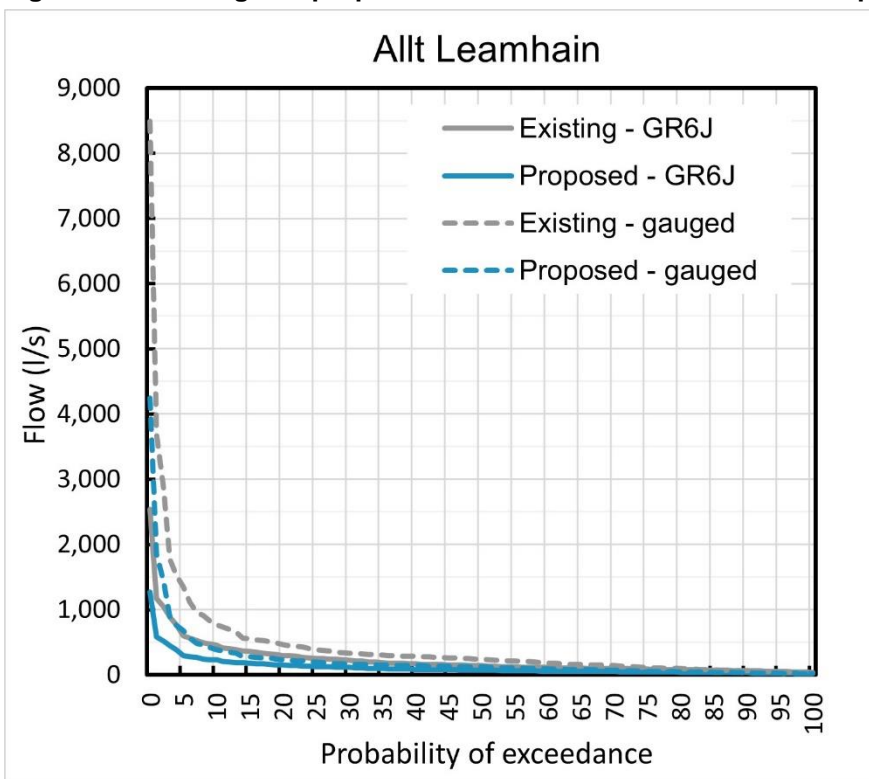
Figure 3.3: Existing and proposed flow duration curve – BH_BHE_update
