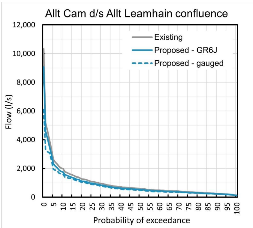
Figure 3.4: Existing and proposed flow duration curve – CA-LEA
