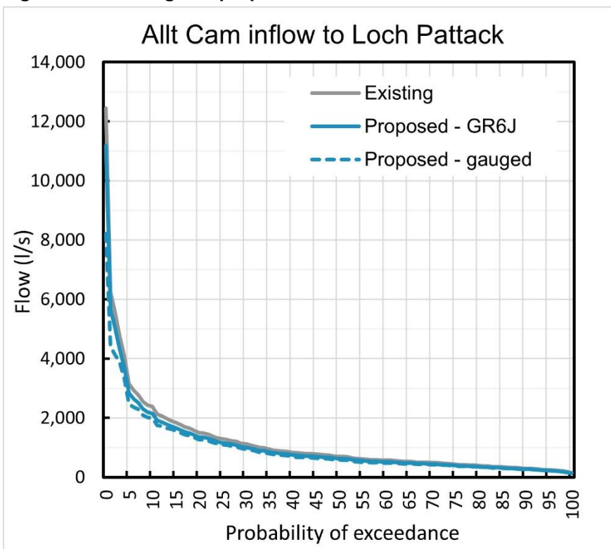
Figure 3.5: Existing and proposed flow duration curve – CA-PAT
