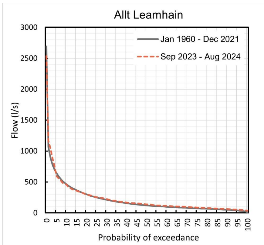
Figure 3.2: Flow Duration Curve adjustment for 2023-2024 period – BH-BHE_update
