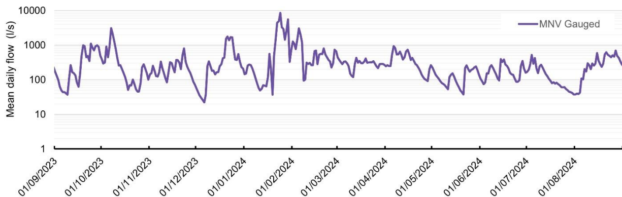
Figure 3.1: Gauged mean daily flow time series – proposed dammed Loch Leamhain catchment
