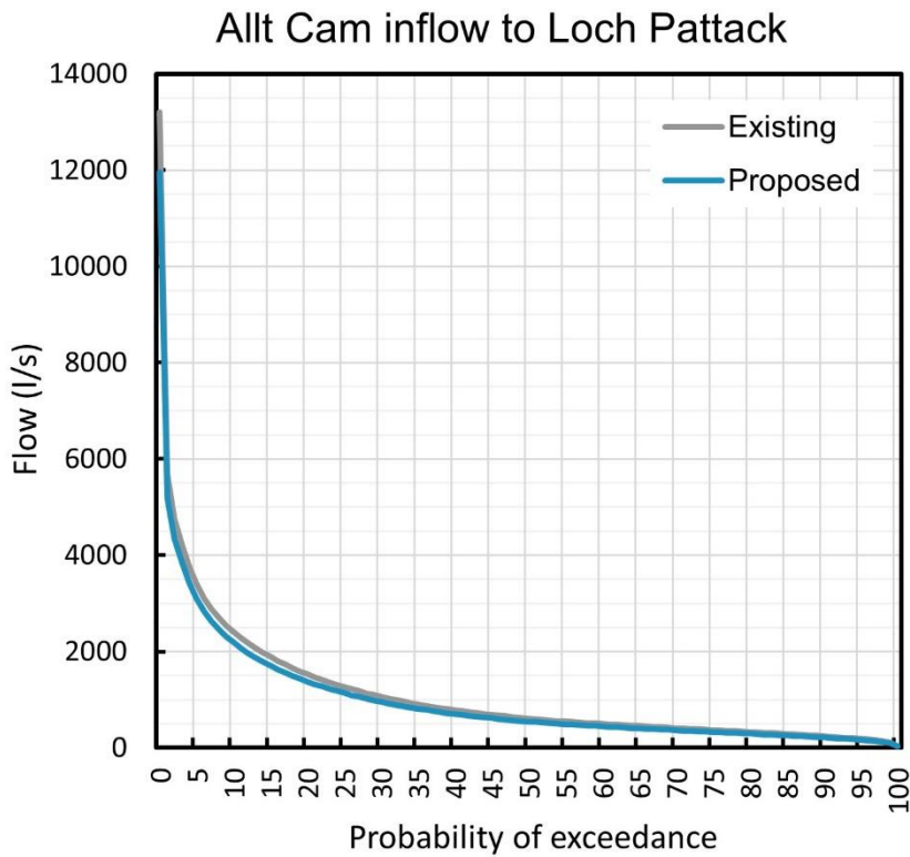
Figure 2.7: Existing and proposed flow duration curve – CA-PAT
