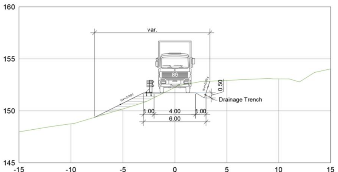
Plate 3.8: Schematic of a Typical Section of Access Track within the Ness Woods SAC
