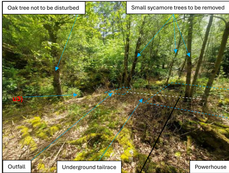
Figure 31 – Powerhouse area
