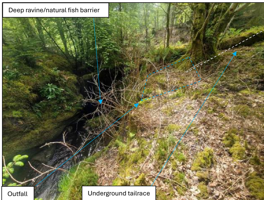
Figure 31 – Tailrace area
