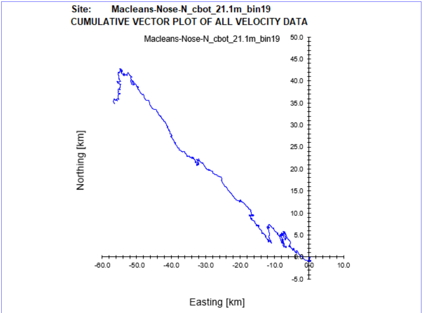
Figure 7. Cumulative Vector Plot of all velocity data from cage bottom cell for ID152.
