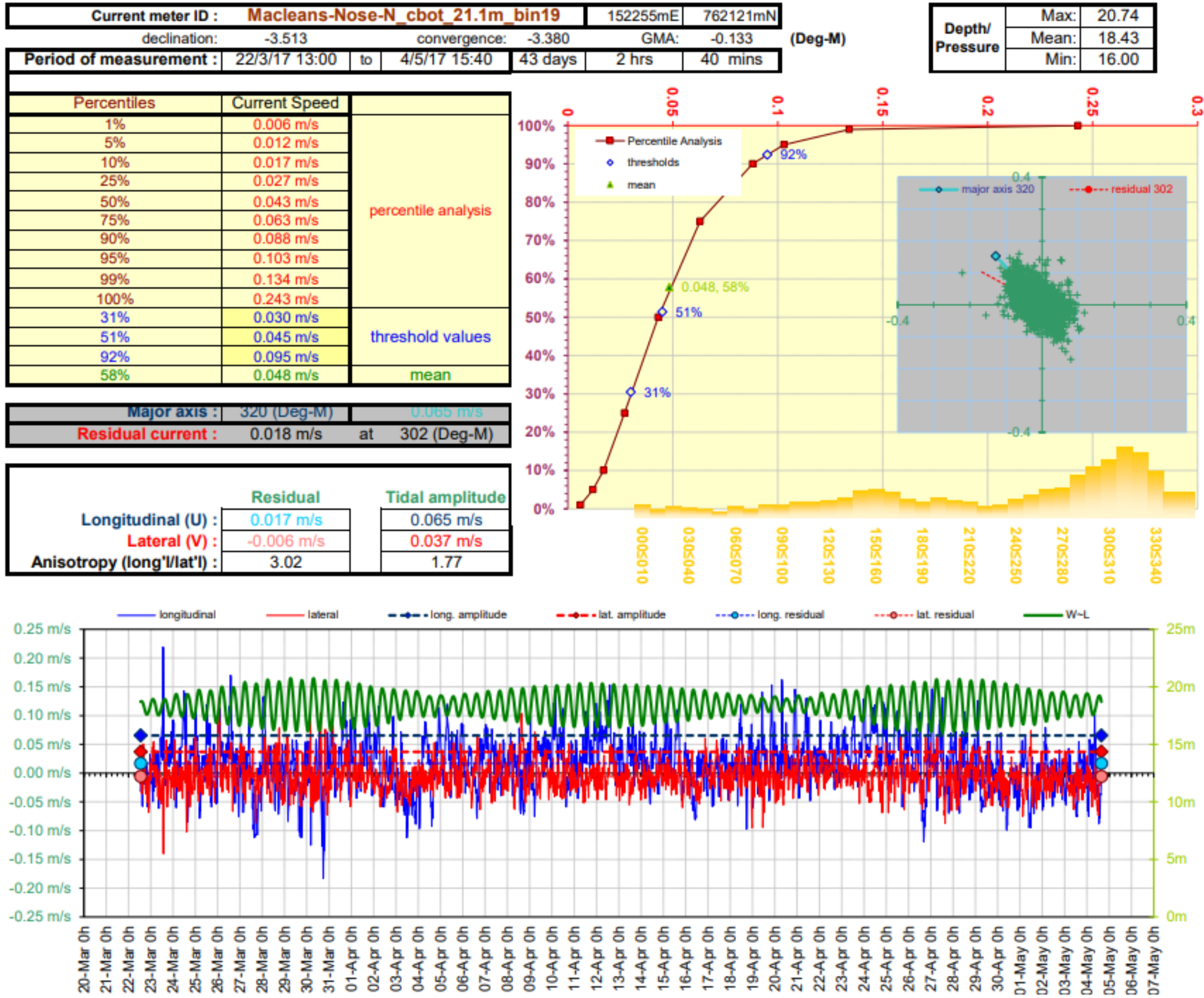
Figure 4. Current Data Summary Sheet for the cage bottom current cell 19, 20.71m from seabed, 22 nd March to 4 th May 2017 inclusive (ID152).
