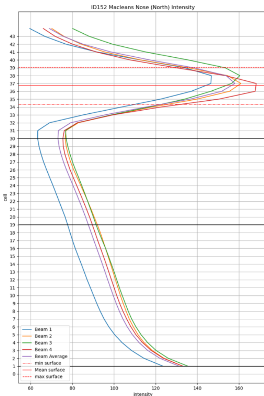
Figure 2. Mean intensity of the ADCP signal for the ID152 dataset plotted by bin number
