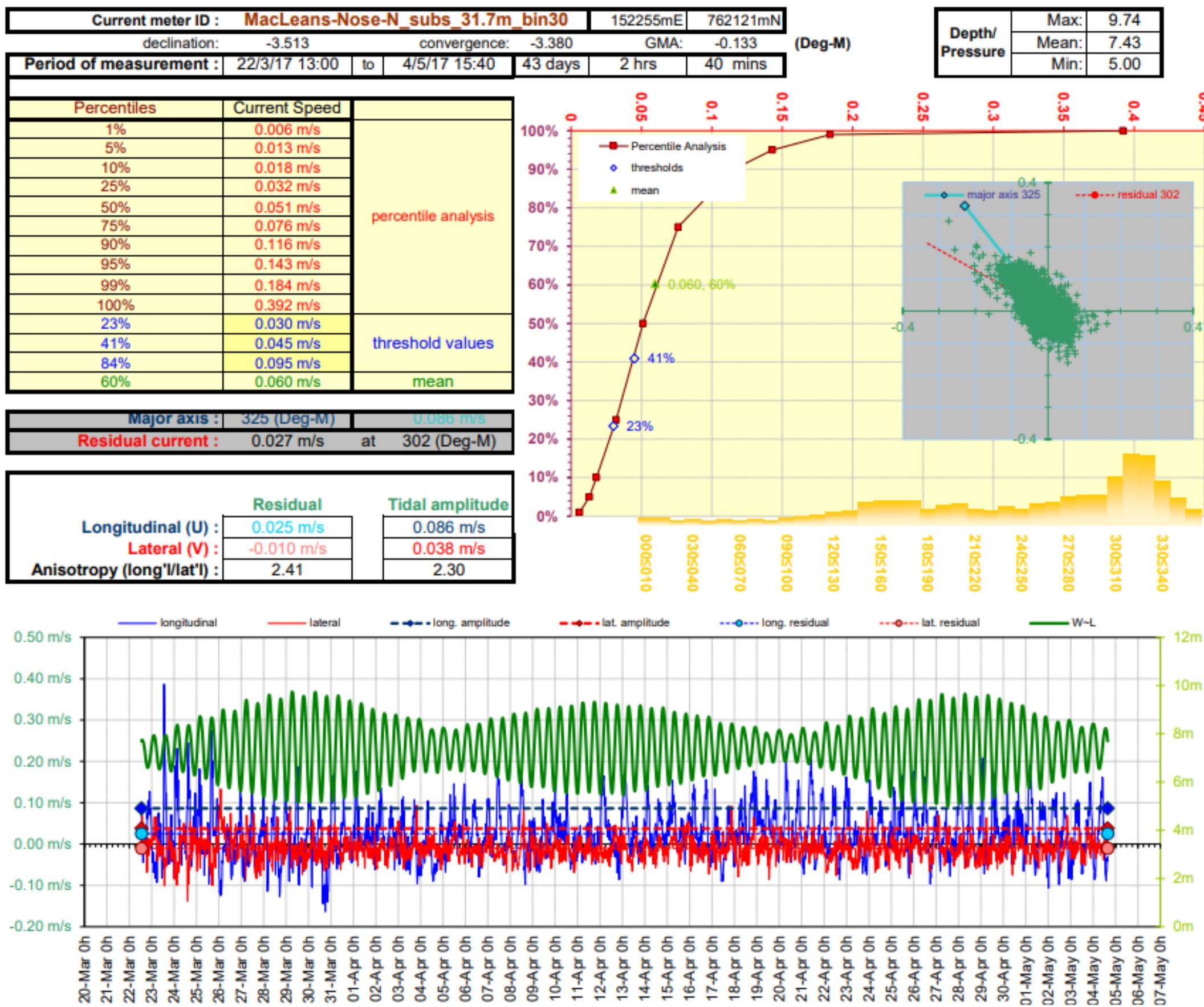
Figure 3. Current Data Summary Sheet for the surface current cell 30, 31.7m from seabed, 22 nd March to 4 th May 2017 inclusive (ID152).
