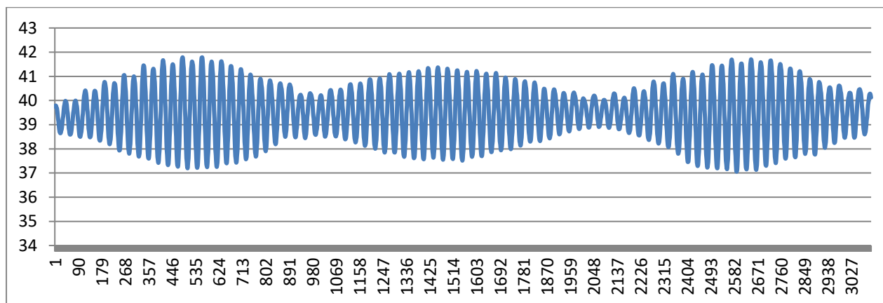
Figure 11. Pressure data from deployment ID152.
