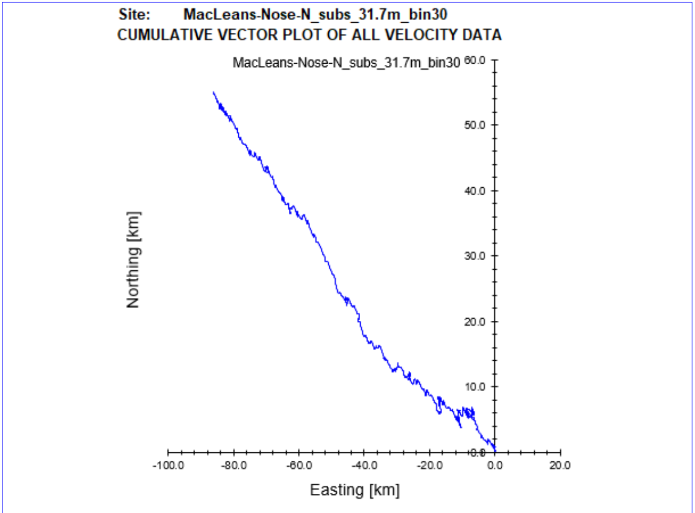
Figure 6. Cumulative Vector Plot of all velocity data from near surface cell for ID152.
