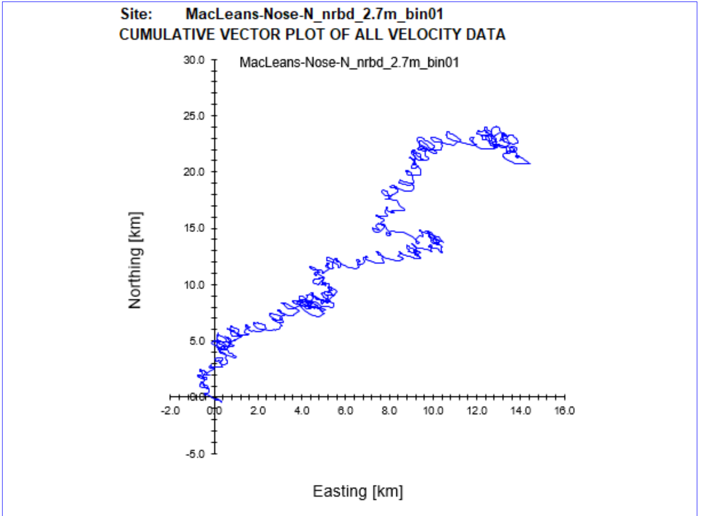
Figure 8. Cumulative Vector Plot of all velocity data from near bottom cell for ID152.
