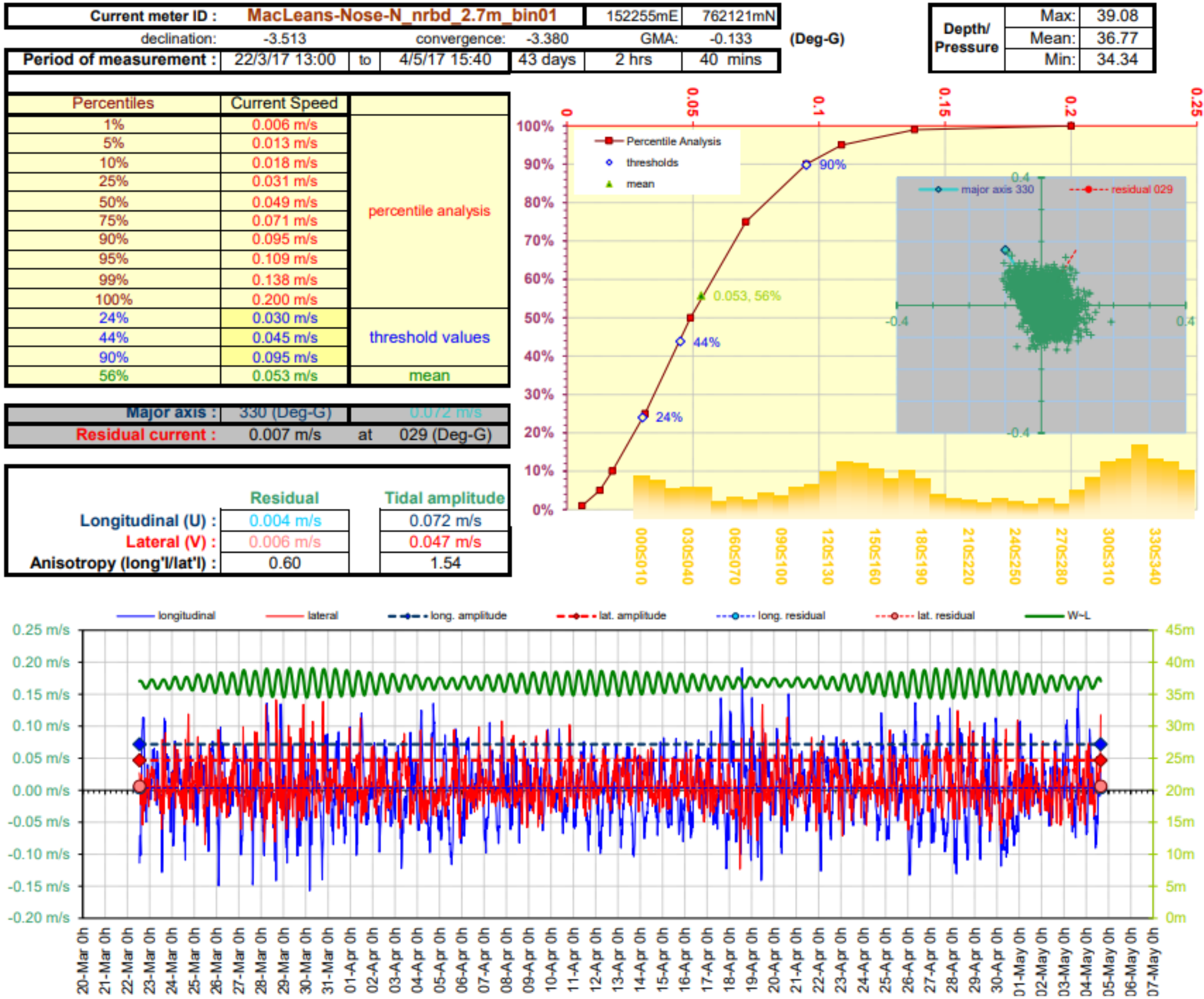
Figure 5. Current Data Summary Sheet for the near bottom current cell 1, 2.71m from seabed, 22 nd March to 4 th May 2017 inclusive (ID152).
