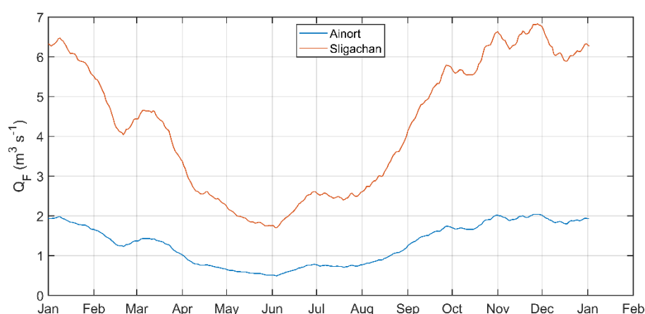
Figure 4. Annual climatological river flows into Loch Ainort and Loch Sligachan used in the modelling.
