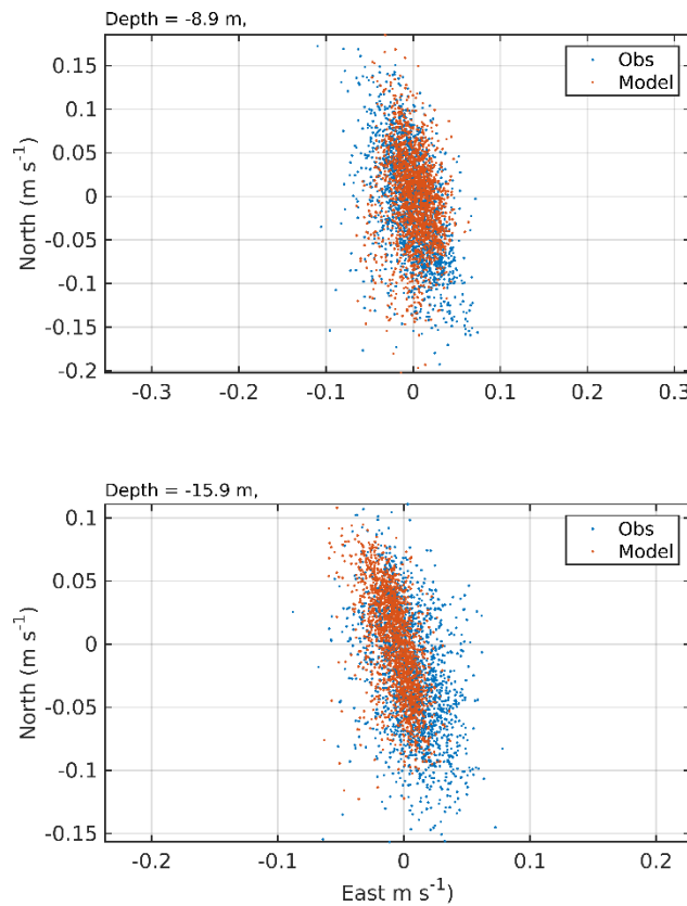
Figure 16. Scatter plot of observed and modelled velocity at the ADCP location from July – September 2018 (ID230) at two depths, 8.9m (top) and 15.9m (bottom). Observed data are in blue, model results in red.
