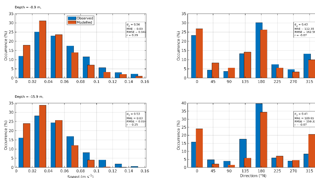
Figure 17. Histograms of observed and modelled current speed (left) and direction (right) at the ADCP location from July – September 2018 (ID230) at two depths, 8.9m (top) and 15.9m (bottom). Observed data are in blue, model results in red.
