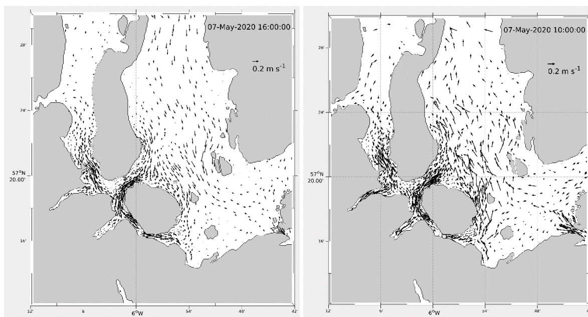
Figure 22. Modelled flood (left) and ebb (right) surface current vectors during spring tides on 7 th May 2020. For clarity, only 25% of the model vectors are shown.
