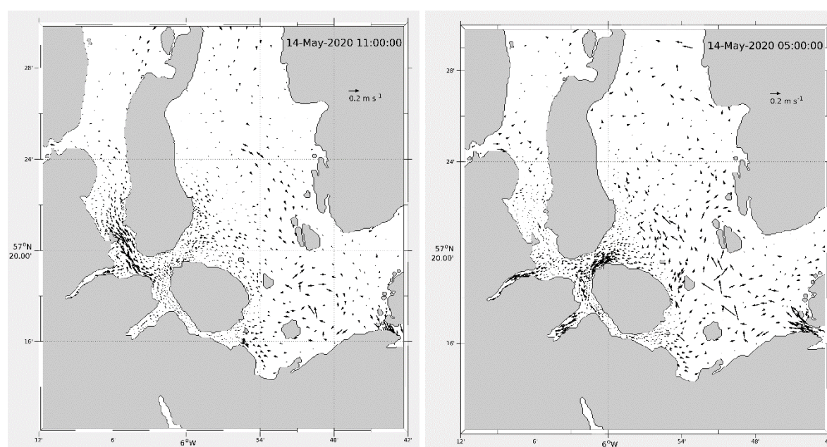
Figure 23. Modelled flood (left) and ebb (right) surface current vectors during neap tides on 14 th May 2020. For clarity, only 25% of the model vectors are shown.
