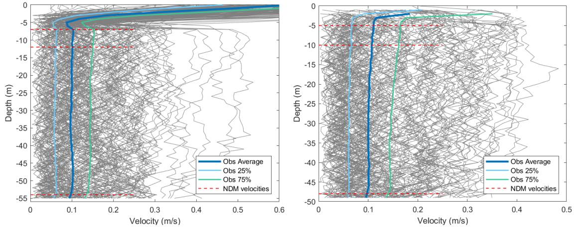
Figure 3.1: Sampled velocity profiles for the hydrographic deployments used in this assessment. Deployment 1 is shown on the left and 2 on the right.
