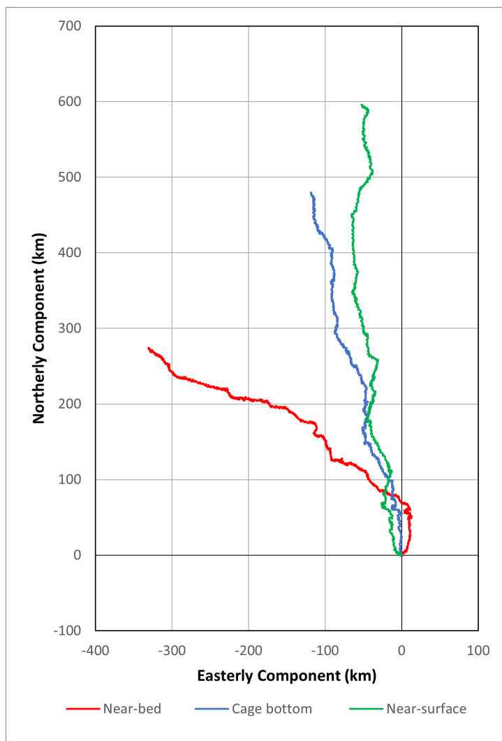
Figure 6.1: Cumulative vector plot of current velocity for all relevant bins.
