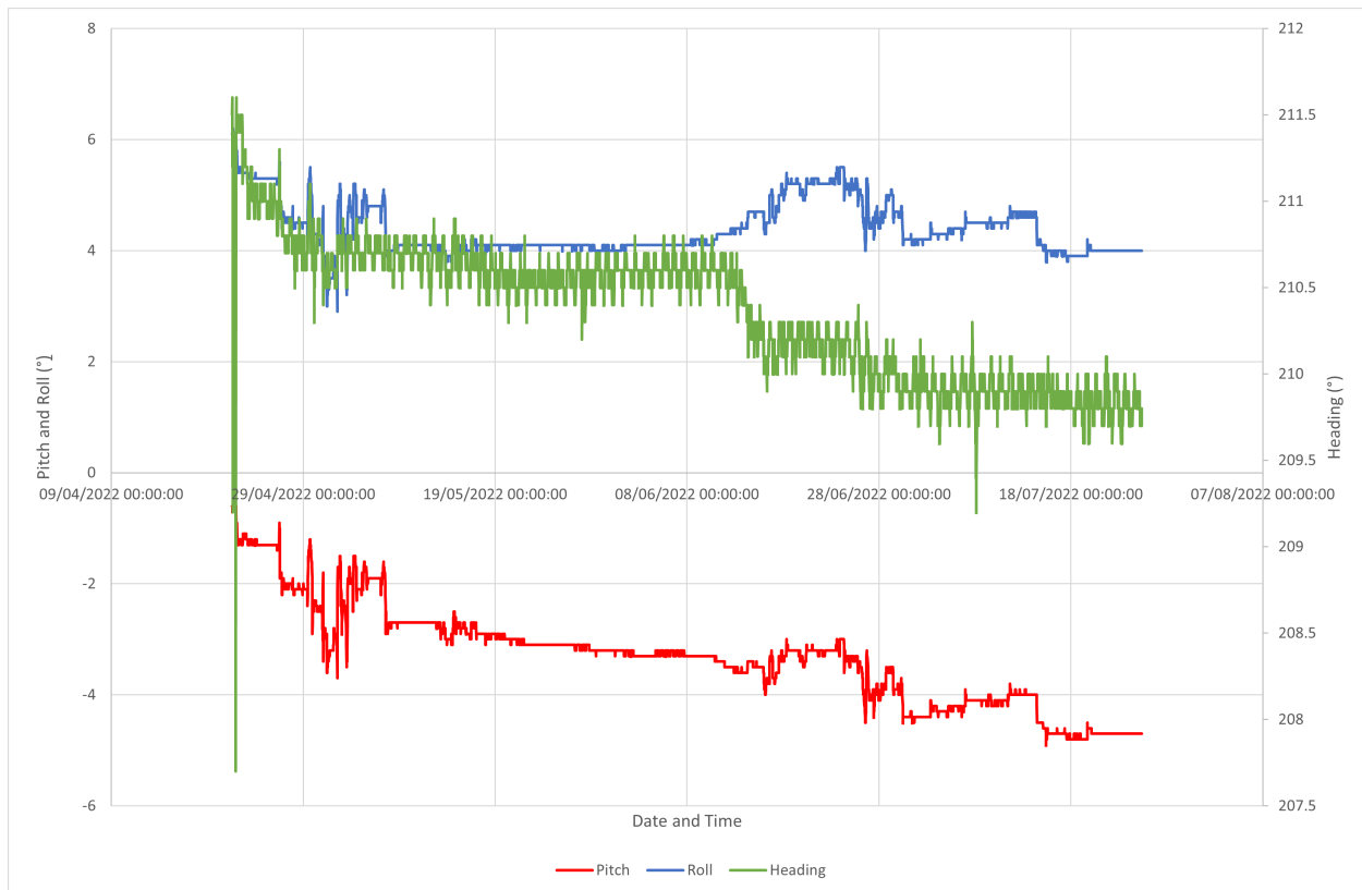
Figure 5.2: Pitch, Roll and Heading data for duration of ADCP deployment.
