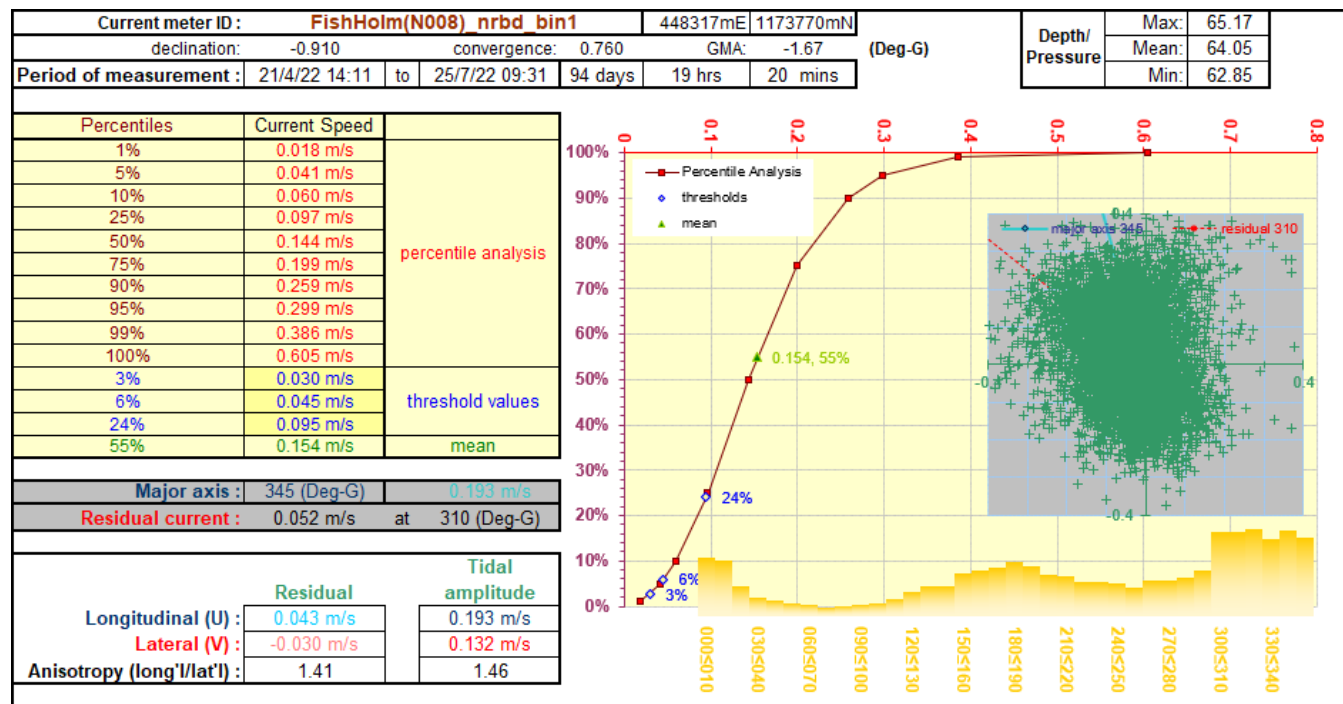
Figure 8.1: Near-bed HG analysis at Fish Holm.
