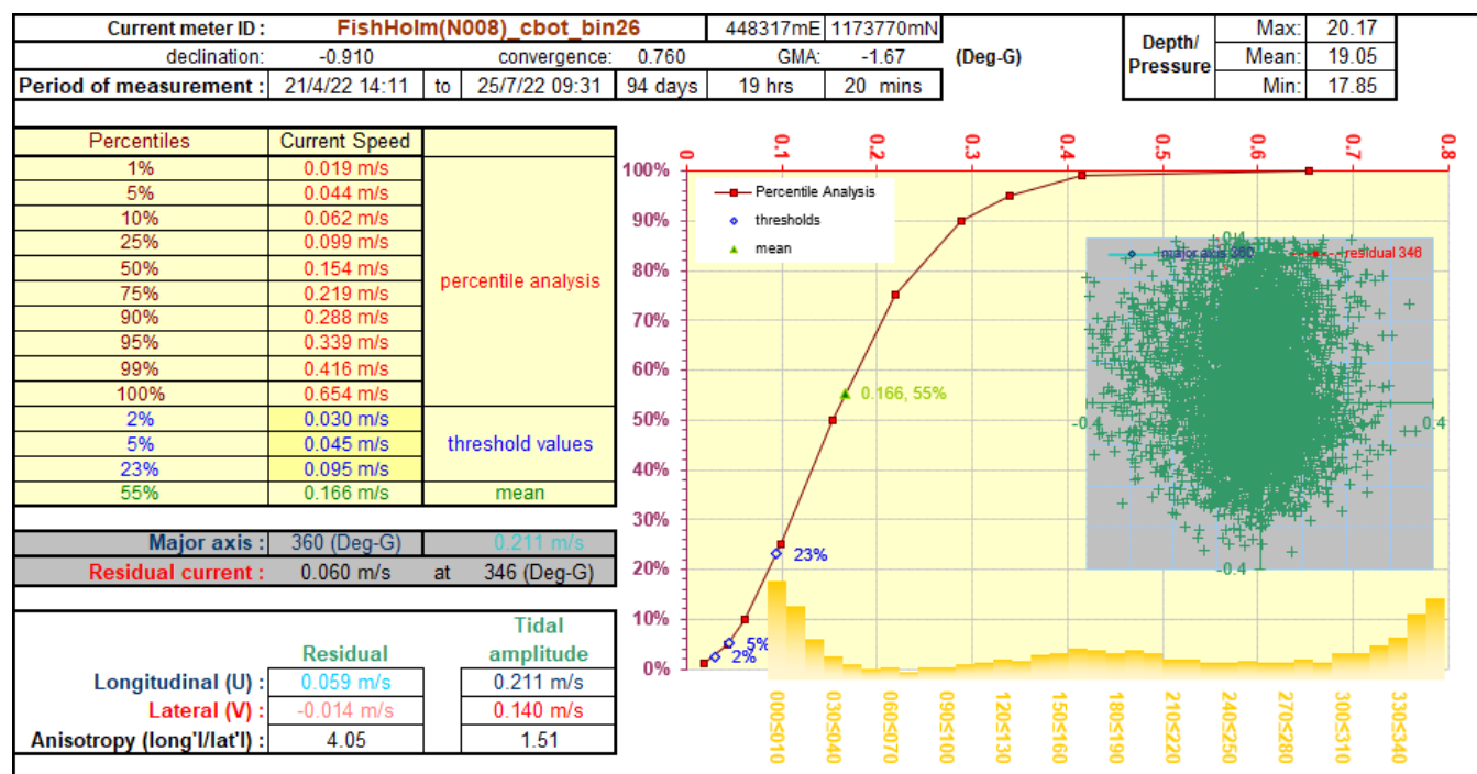
Figure 8.2: Cage-bottom HG analysis at Fish Holm.
