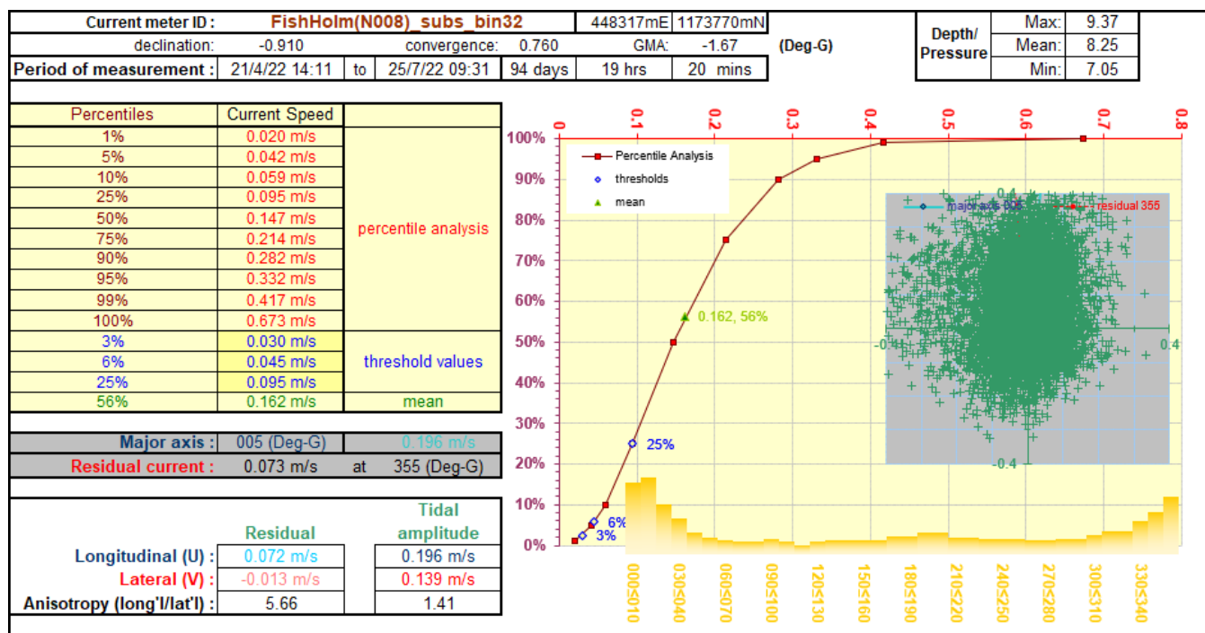
Figure 8.3: Sub-surface HG analysis at Fish Holm.
