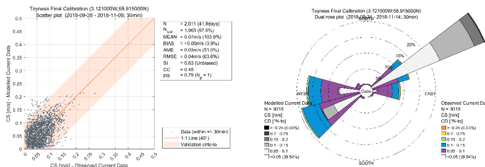
Figure A.8.9 Scatter and rose plot of observed vs model total current speed at Toyne (orange shading denotes SEPA’s calibration standards)
