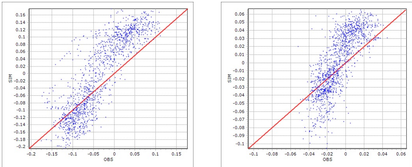
Figure 2.24 Scatter plot comparison of 3D model simulation results and observations at Toyneess for u velocity (m/s left) and v velocity (m/s right) for the period 28 th Sept -8 th November 2018
