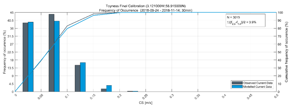
Figure A.8.11 Overlaid frequency distributions of observed and modelled total current speed at Toyne
