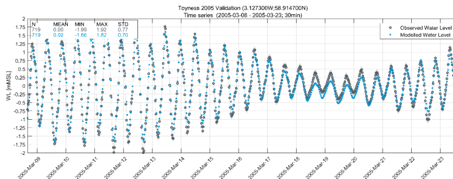
Figure A.8.14 Time series plot of observed vs. model total water level at Toyneess for 2005 validation period
