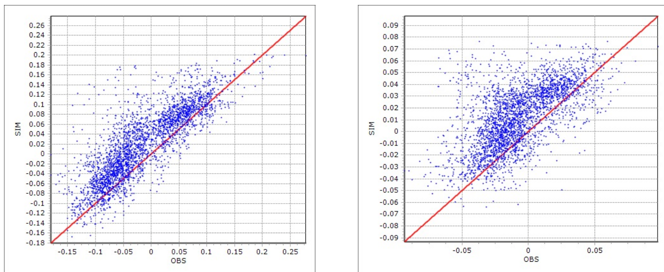
Figure 2.22 Scatter plot comparison of 2D model simulations results and observations at Toyneys for u velocity (m/s left) and v velocity (m/s right) for the period 28 th Sept -8 th November 2018
