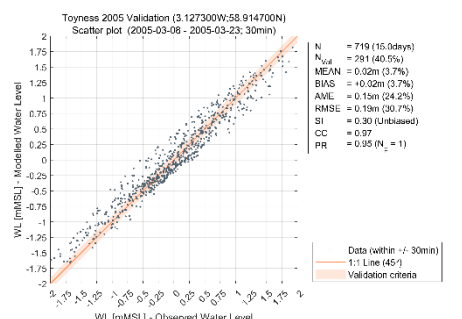
Figure A.8.13 Scatter plot of observed vs. model total water level at Toyneess for 2005 validation period (orange shading denotes SEPA's calibration standards)
