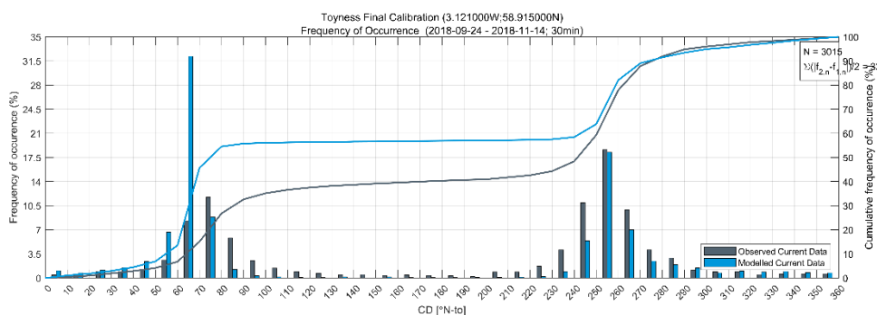
Figure A.8.10 Overlaid frequency distributions of observed and modelled total current direction (towards) at Toyne
